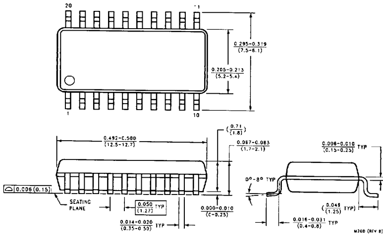
Small Outline Package (SJ) Order Number DM74ALS373SJ NS Package Number M20D
