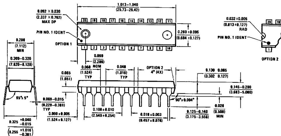
Molded Dual-In-Line Package (N) Order Number DM74ALS373N NS Package Number N20A
