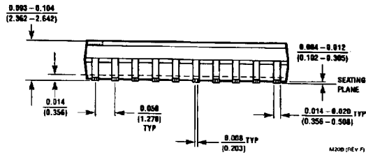
S.O. Package (M) Order Number DM74ALS373WM NS Package Number M20B
