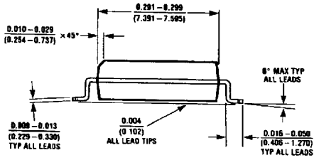
S.O. Package (M) Order Number DM74ALS373WM NS Package Number M20B
