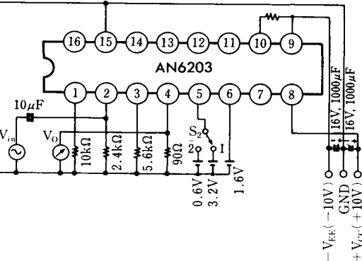
Test Circuit 3 ( V_{Omax,2} , THD_2 , V_{no2} , V_{MO2} )
