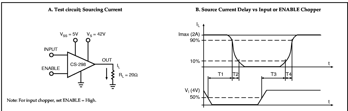
Figure 1. Switching Times
