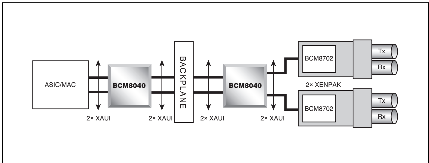
Dual Independent XAUI Cross-Link Application Diagram
