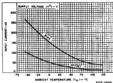
Fig. 3 - Input current ( I_{iO} , I_{iB} ) vs. temperature.
