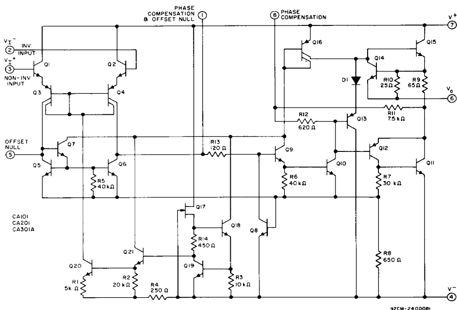
Fig. 2 - Schematic diagram.
