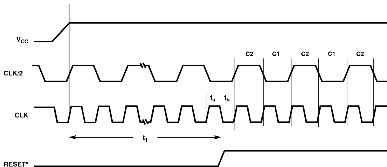
Figure 6-1. Reset Timing
