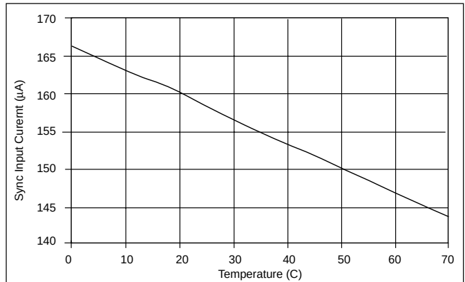
Figure 29: SYNC Input Current vs Temperature ( V_{\text{SYNC}} = 2.4\text{V} ).
