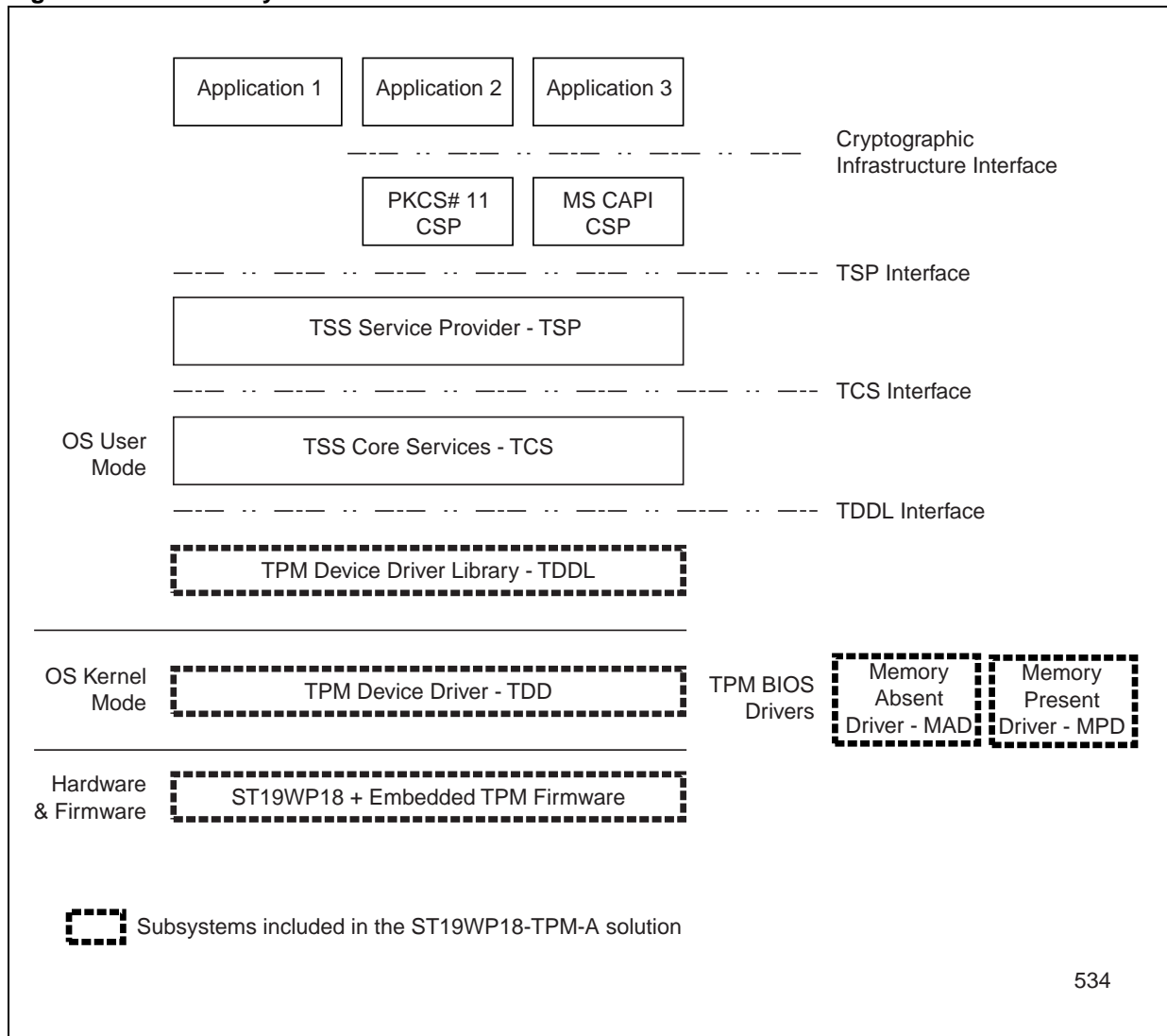
Figure 3. Software Layers
