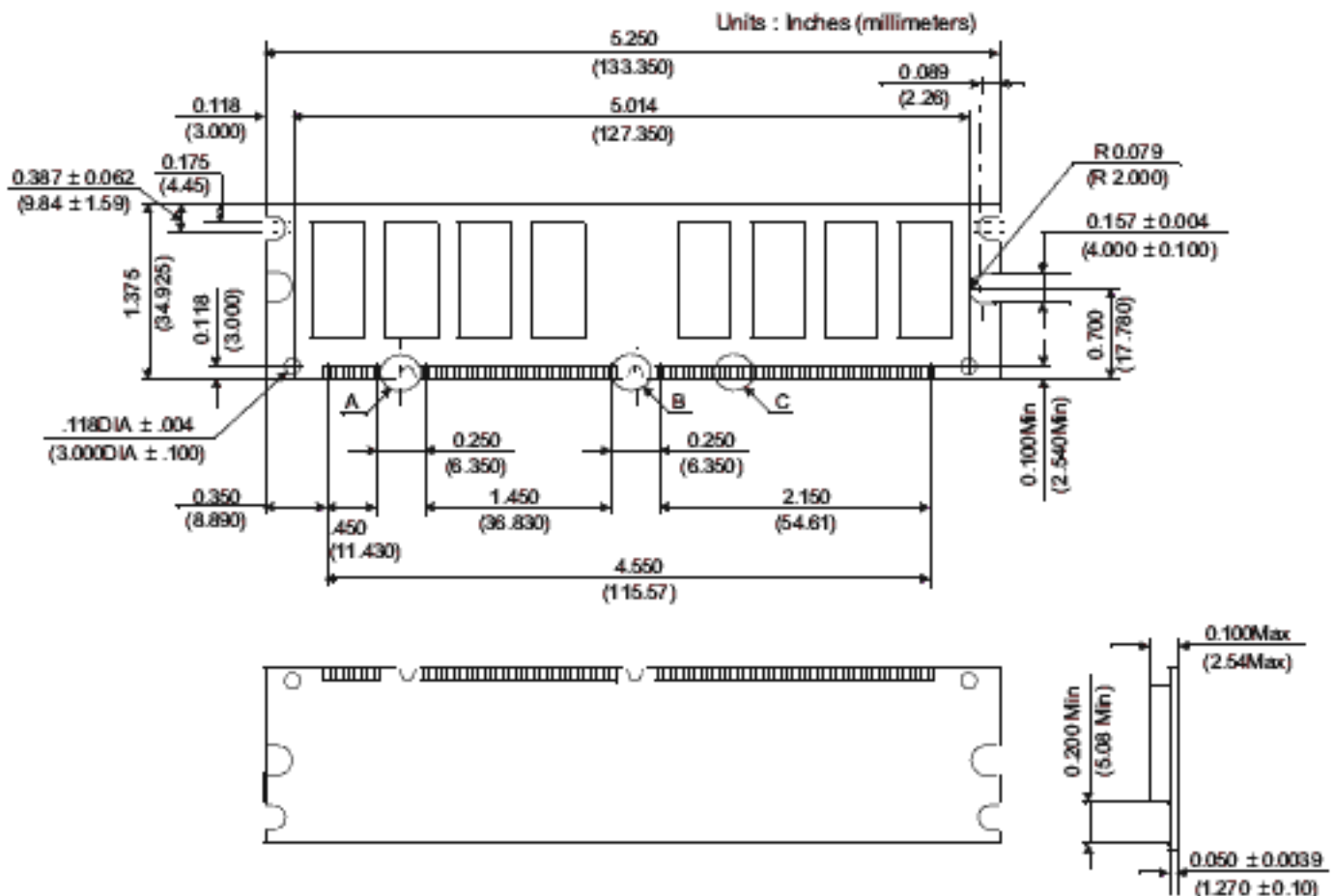
Figure 1: KVR133X64C3SS/256 168-Pin SDRAM Module
