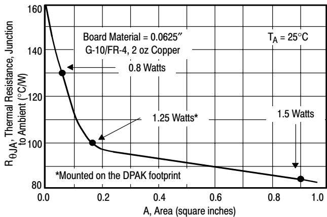
Figure 17. Thermal Resistance versus Collector Pad Area for the SOT-223 Package (Typical)
