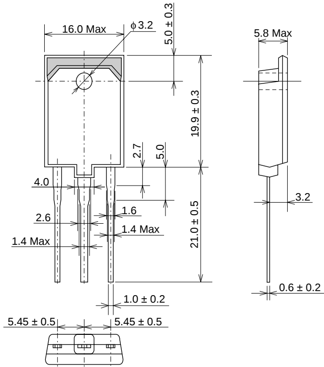
Package Outline
