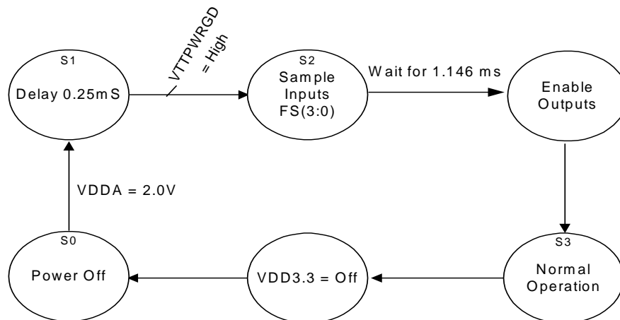
Figure 10. Clock Generator Power-up/Run State Diagram
