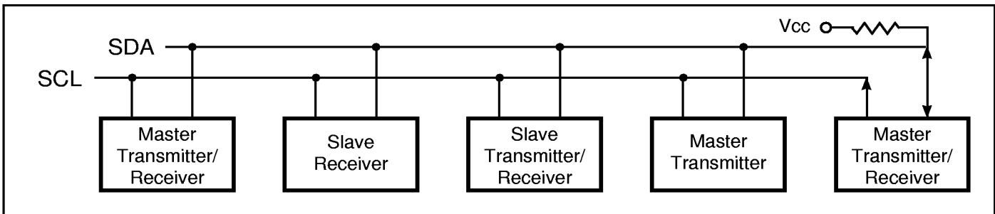
Figure 1. Typical System Bus Configuration
