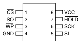
8-lead SOIC
