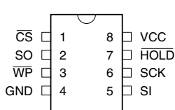
8-lead PDIP
