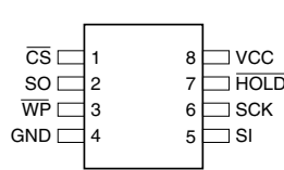
8-lead SOIC
