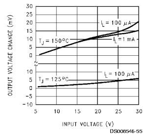
Line Regulation
