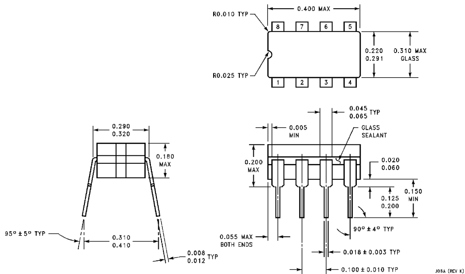
Ceramic Dual-In-Line Package (J) Order Number LP2951CJ, LP2951ACJ, LP2951J, LP2951J/883 or 5962-3870501MPA NS Package Number J08A
