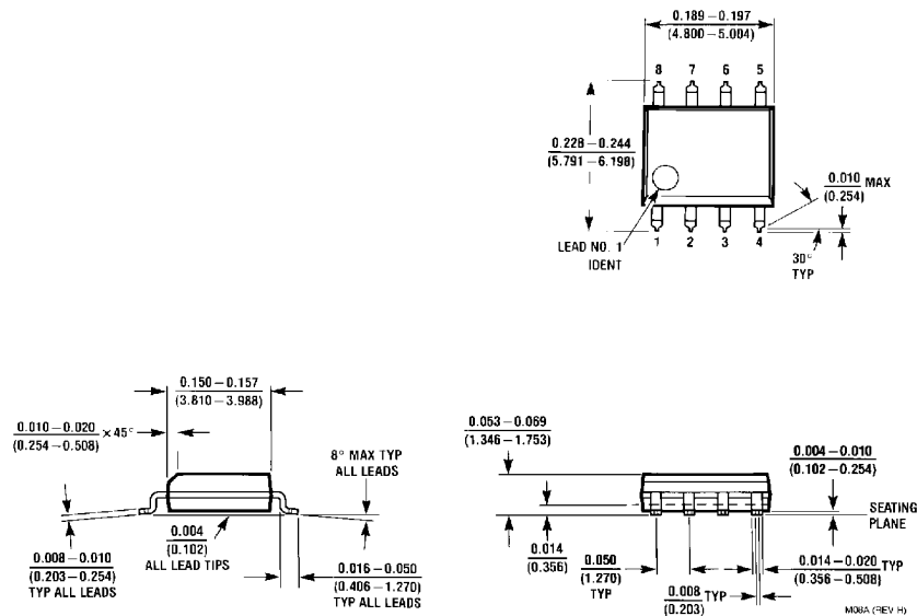
Surface Mount Package (M) Order Number LP2951ACM, LP2951CM, LP2951ACM-3.0, LP2951CM-3.0, LP2951ACM-3.3 or LP2951CM-3.3 NS Package Number M08A
