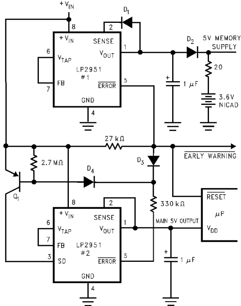
Regulator with Early Warning and Auxiliary Output
