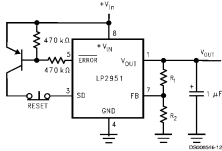
Latch Off When Error Flag Occurs
