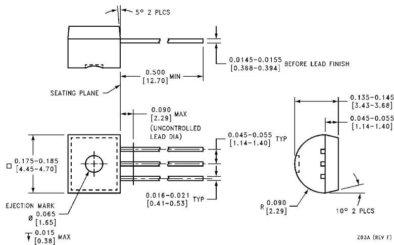
Molded TO-92 Package (Z) Order Number LP2950ACZ-3.0 or LP2950CZ-3.0, LP2950ACZ-3.3, LP2950CZ-3.3, LP2950ACZ-5.0 or LP2950CZ-5.0 NS Package Number Z03A
