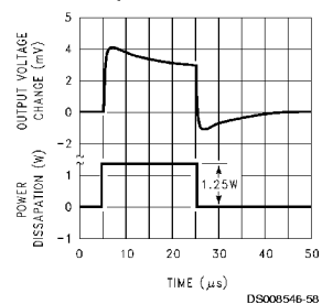
Thermal Response
