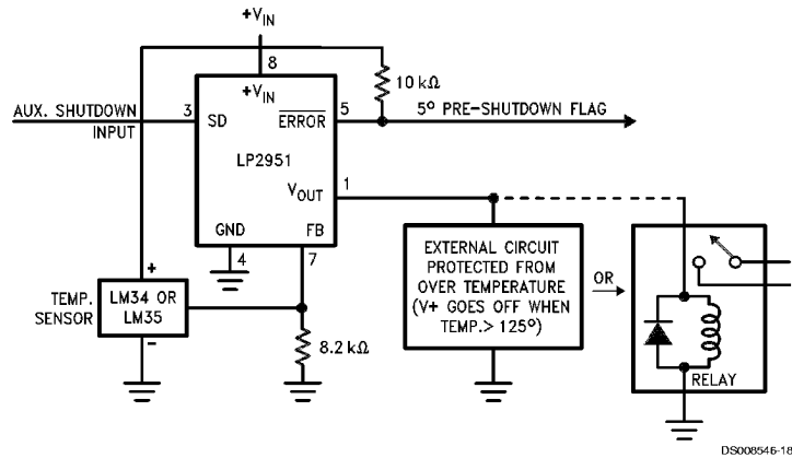
System Overtemperature Protection Circuit
