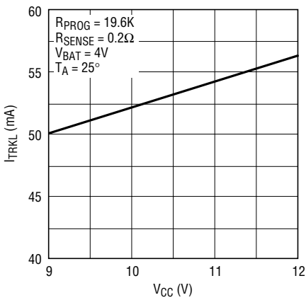
Trickle Charge Current vs V_{CC}
