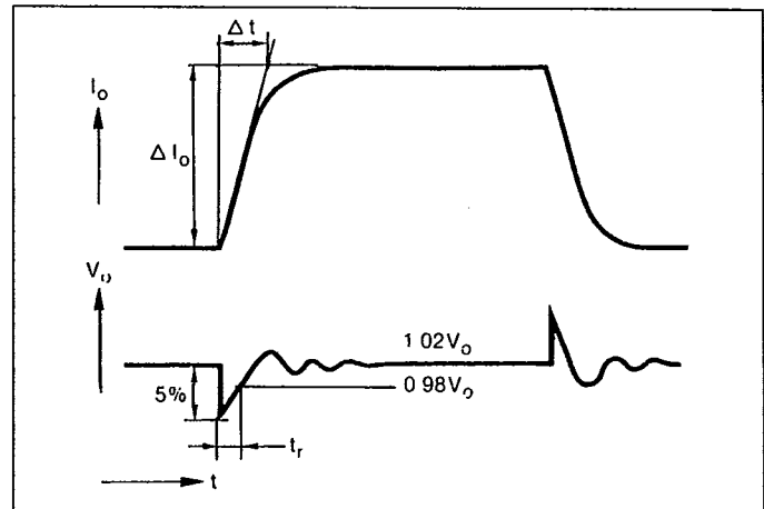
Fig. 5 \Delta I_o = 0.8 \times I_{o, \text{nom}} , \Delta t = 100\mu s .
