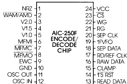
DIP PACKAGE
