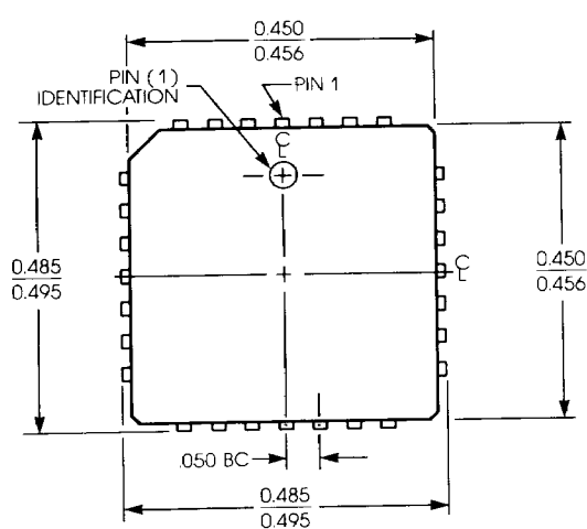
28-Lead Plastic Surface Mount Package
