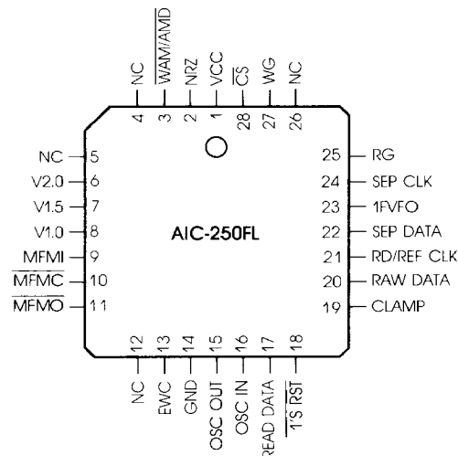
QUAD PLCC PACKAGE
