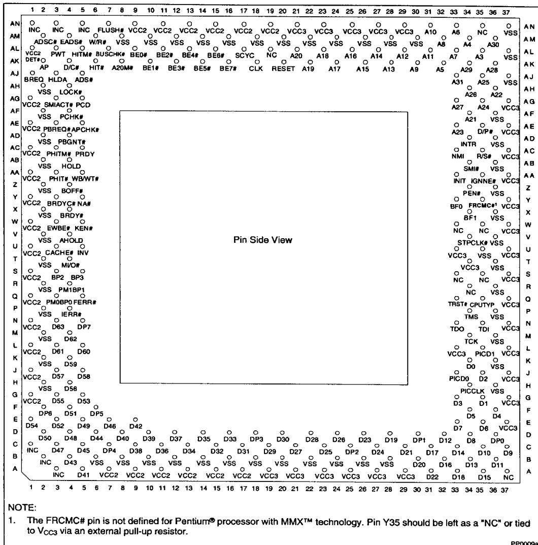
Figure 3. Pentium® Processor with MMX™ Technology SPGA and PPGA Package Pinout (Pin Side View)
