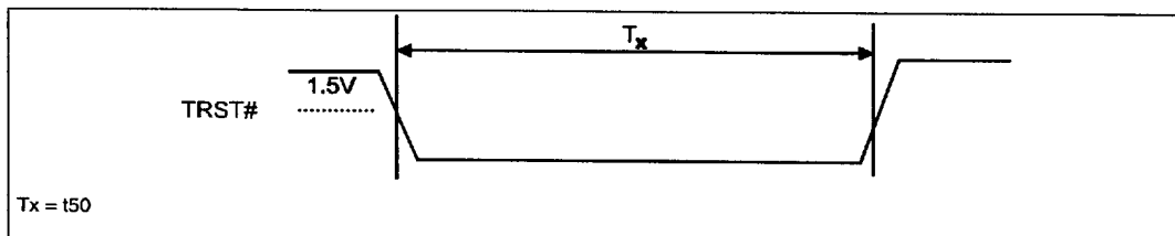
Figure 10. Test Reset Timings
