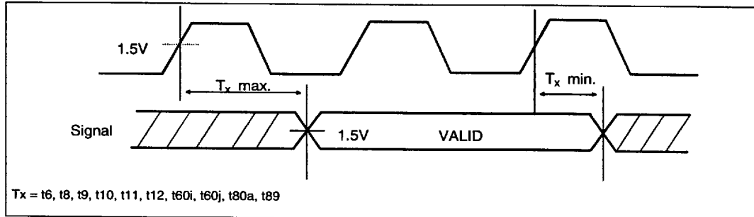
Figure 5. Valid Delay Timings
