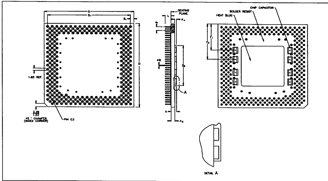
Figure 13. PPGA Package Dimensions
