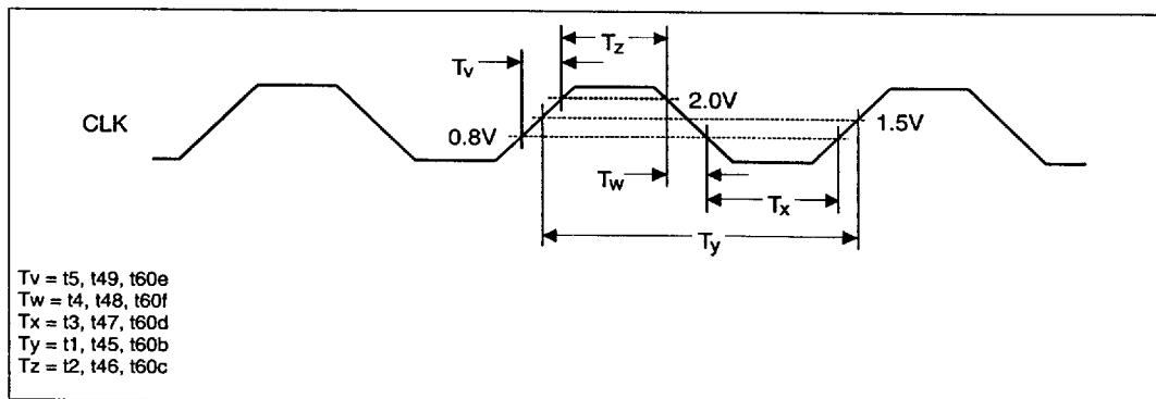
Figure 4. Clock Waveform
