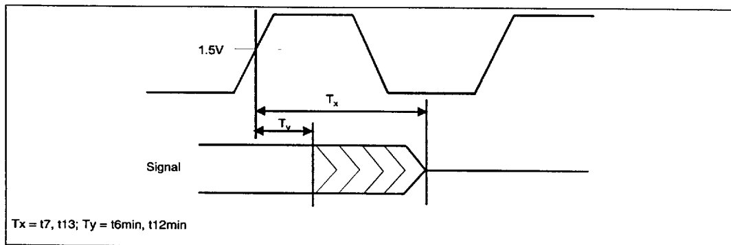
Figure 6. Float Delay Timings
