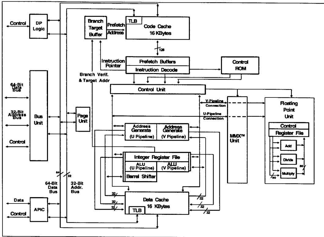
Figure 1. Pentium® Processor with MMX™ Technology Block Diagram
