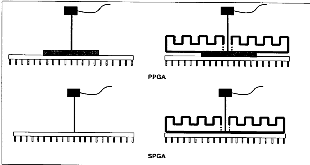
Figure 14. Technique for Measuring T_c on PPGA and SPGA Packages
