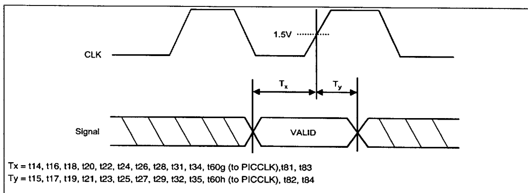
Figure 7. Setup and Hold Timings
