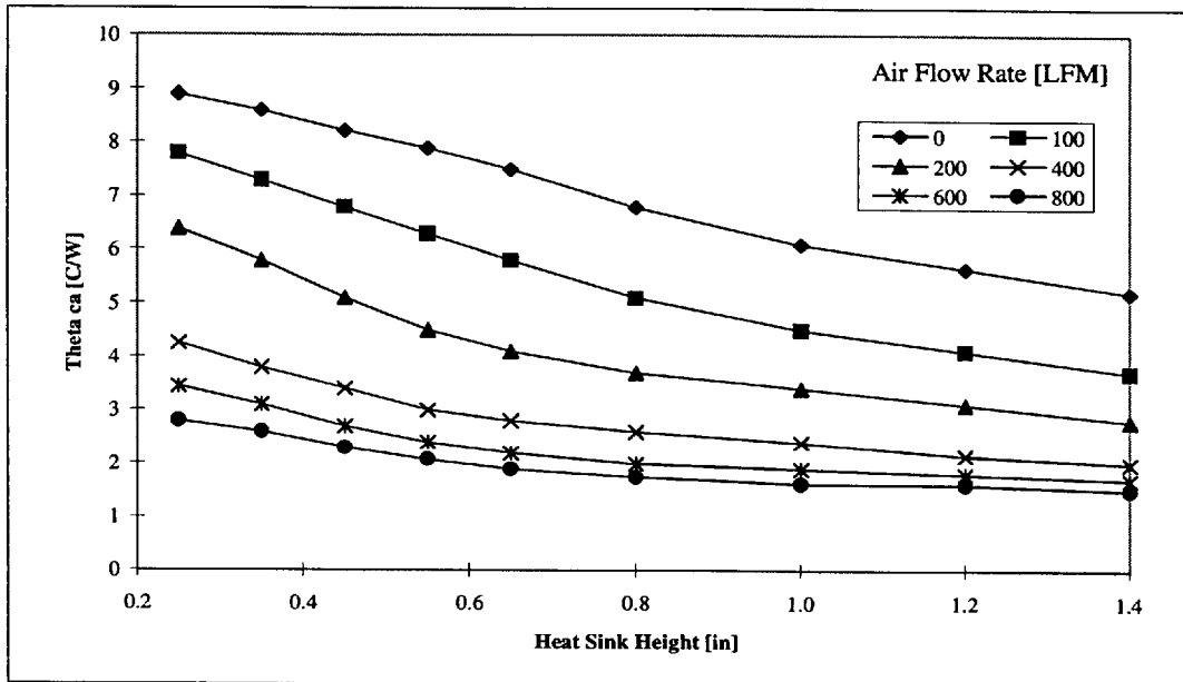
Figure 16. Thermal Resistance vs. Heatsink Height, PPGA Packages
