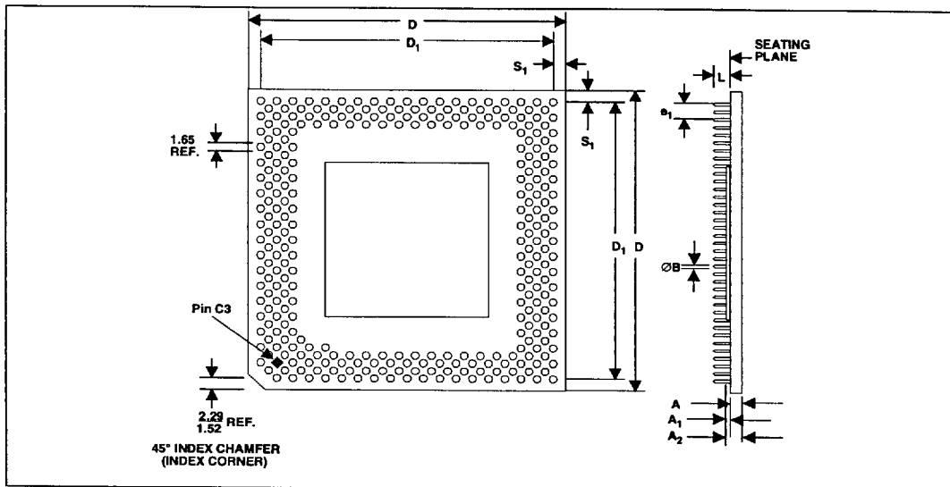
Figure 12. SPGA Package Dimensions
