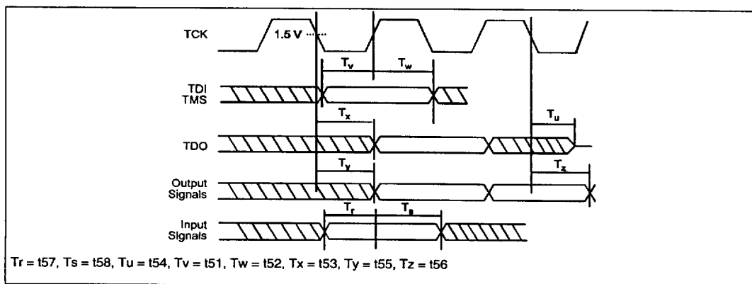
Figure 9. Test Timings
