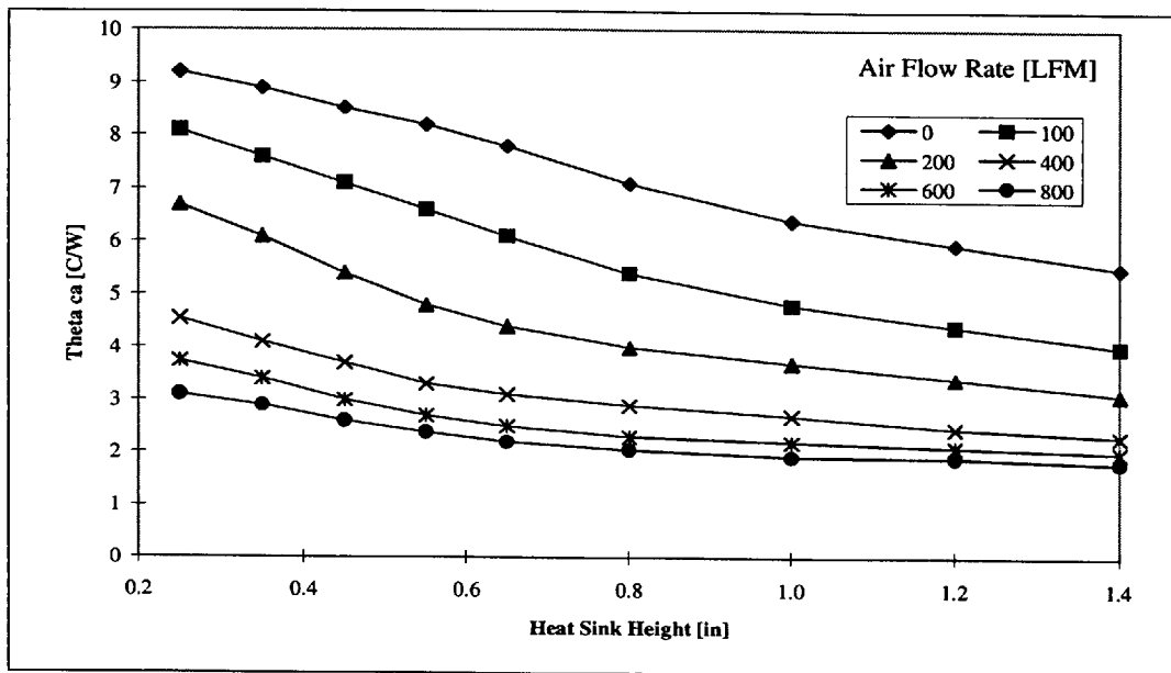
Figure 15. Thermal Resistance vs. Heatsink Height, SPGA Packages
