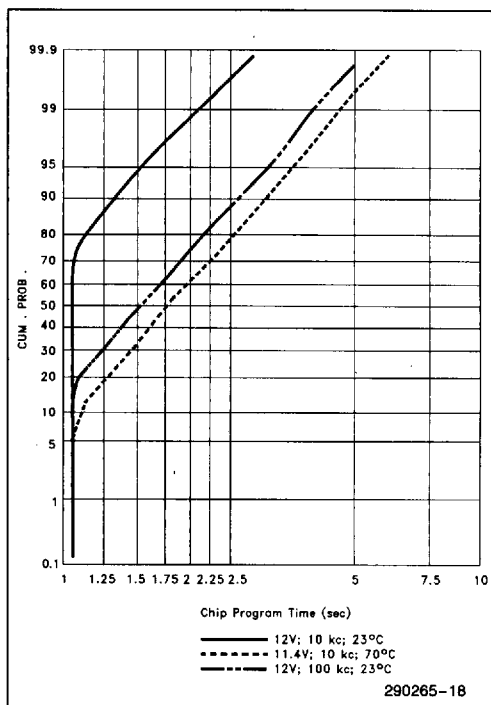
Figure 8. 28F512 Typical Programming Capability
