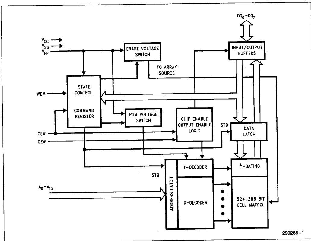
Figure 1. 28F512 Block Diagram
