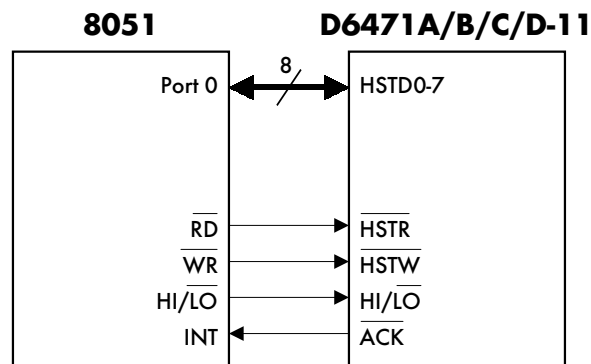
Figure 4. D6471A/B/C/D - Host Interface
