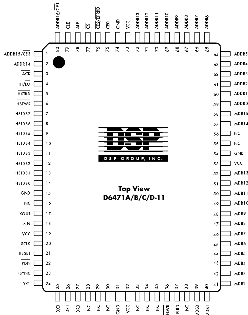
Figure 2. D6471A/B/C/D-11 Pin Diagram
