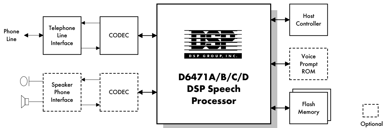
Figure 1. D6471A/B/C/D System Block Diagram
