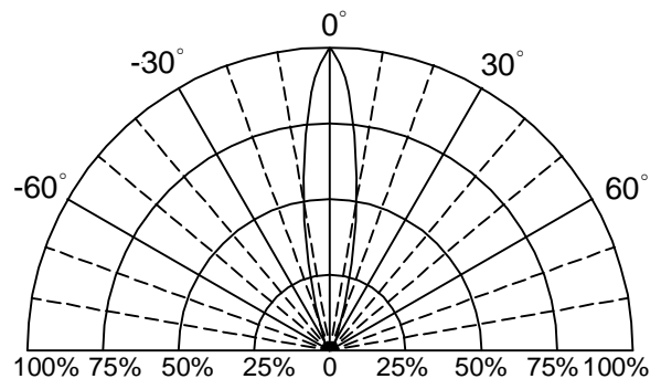
Fig.6 Directivity Radiation
