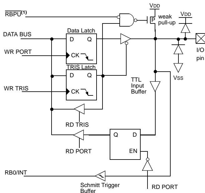
FIGURE 3-3: BLOCK DIAGRAM OF RB0 PIN
