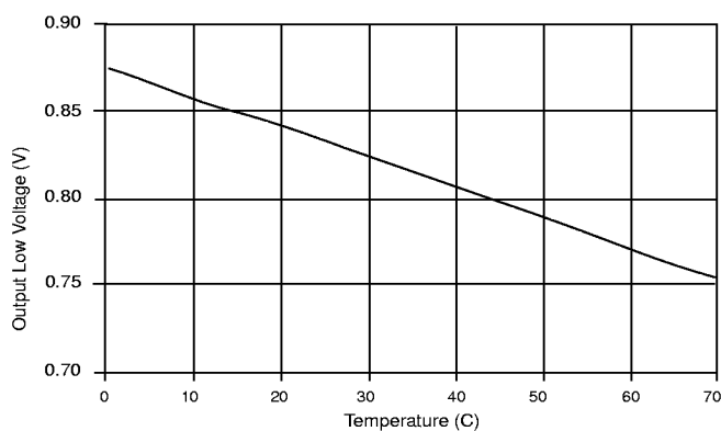
Figure 34: Error Amplifier Output Low Voltage (500µA) vs Temperature.
