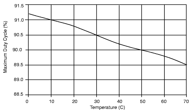
Figure 23: Oscillator Maximum Duty Cycle vs Temperature.
