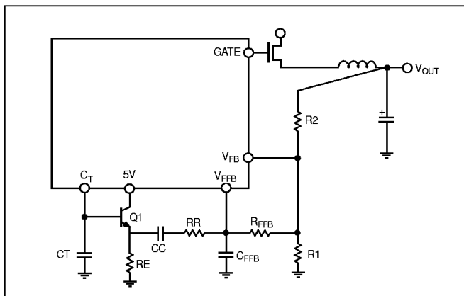
Figure 4. Artificial ramp components CC, C_{FFB} , RR and R_{FFB} must be provided for each channel if duty cycle for that channel exceeds 50%. Q1 and RE are common to both channels. DC voltage is shown supplied to V_{FFB} through the V_{FB} resistor divider.
