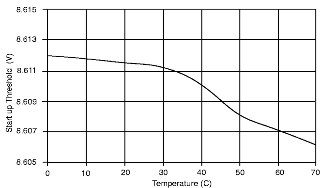
Figure 42: V_{IN} Start-up Threshold vs Temperature.
