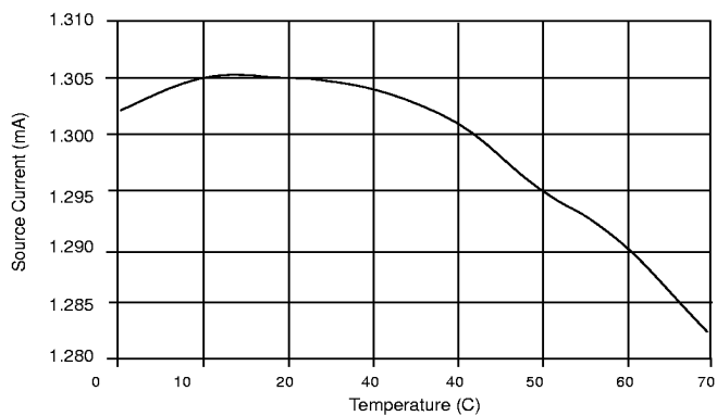
Figure 30: Error Amplifier Source Current vs Temperature.
