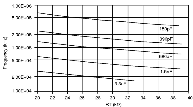
Figure 22: Oscillator Frequency vs R T , C T (V IN = 12V, T = 25°C)
