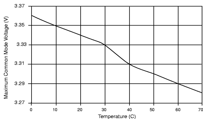
Figure 35: PWM Comparator Maximum Common Mode Input Voltage vs Temperature.
