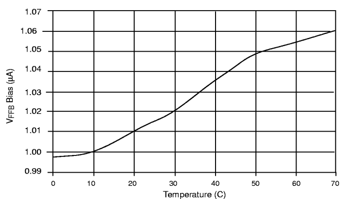
Figure 37: V_{FFB} Bias Current vs Temperature.
