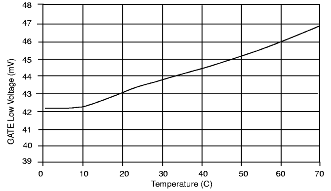
Figure 39: GATE low voltage (20mA) vs Temperature.
