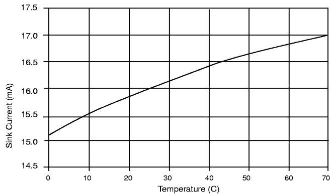
Figure 33: Error Amplifier Sink Current vs Temperature.
