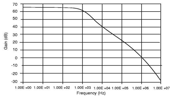
Figure 29: Error Amplifier Gain vs Frequency.
