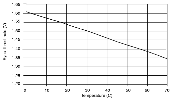
Figure 26: SYNC Threshold vs Temperature.
