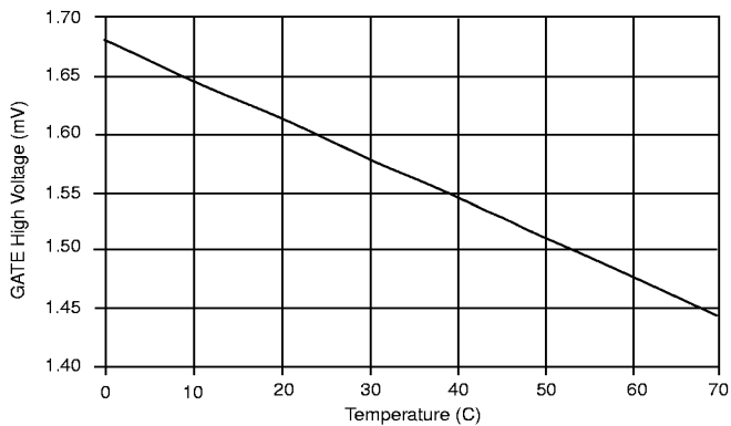
Figure 41: GATE High Voltage (100mA) vs Temperature.
