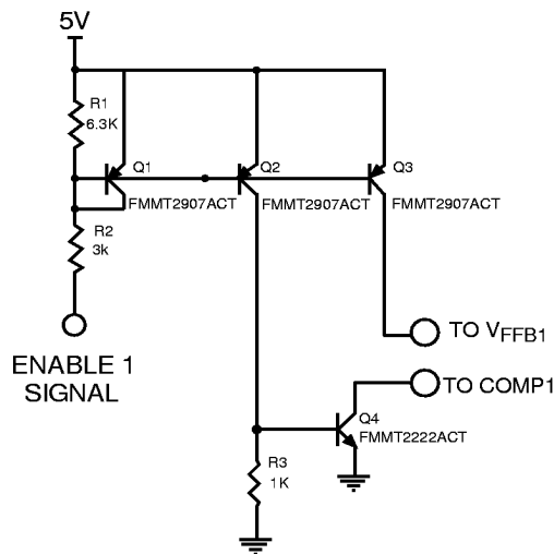
Figure 13: An external circuit can be built to provide an enable function for channel 1. The circuit shown above connects to the V_{FB1} and COMP1 pins as indicated. If the ENABLE1 signal is left floating or is pulled high, channel 1 is enabled. If the ENABLE1 pin is pulled below 1V, Q1 will conduct, and mirror Q3 pulls V_{FFB1} up at the same time as Q2 and Q4 pull COMP1 low. This will force GATE1 to go low and turn off the switch FET. The circuit above will provide about 1mA of additional drive to the V_{FFB1} pin components. This additional current must be sufficient to pull V_{FFB1} up to about 1V in order to guarantee GATE1 is held low.
