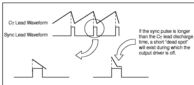
Figure 2: Sync pulse duration vs. C_T lead discharge time.
