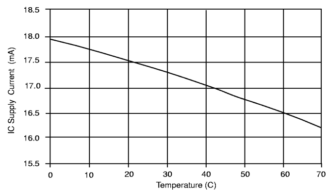
Figure 47: IC Supply Current vs Temperature. No Load on GATE pins. R_T = 27k , C_T = 330pF
