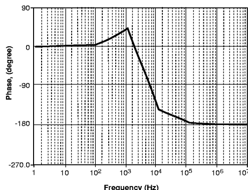
Figure 10: Bode plot of phase response for compensated voltage mode system.
