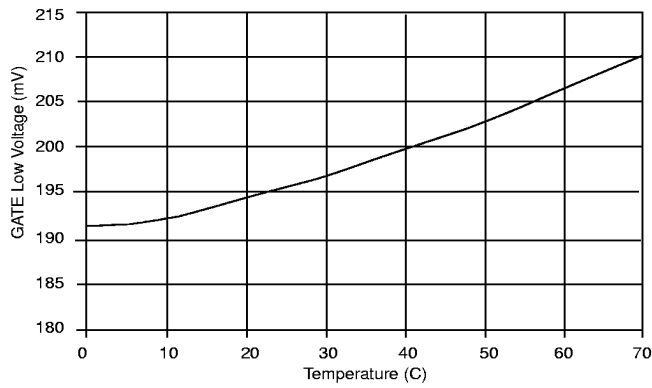
Figure 40: GATE Low Voltage (100mA) vs Temperature.
