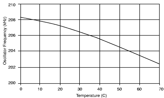
Figure 24: Oscillator Frequency vs Temperature. C T = 330pF, R T = 27k
