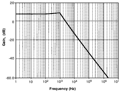
Figure 7: Bode plot of gain response for V_{OUT}/V_{CONTROL}
