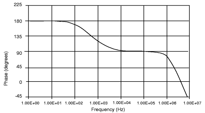
Figure 32: Error Amplifier Phase vs Frequency.
