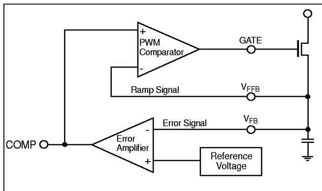
Figure 1: V^2 control diagram.
