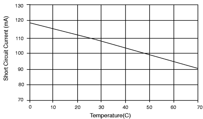
Figure 21: V REF Short Circuit Current vs Temperature.
