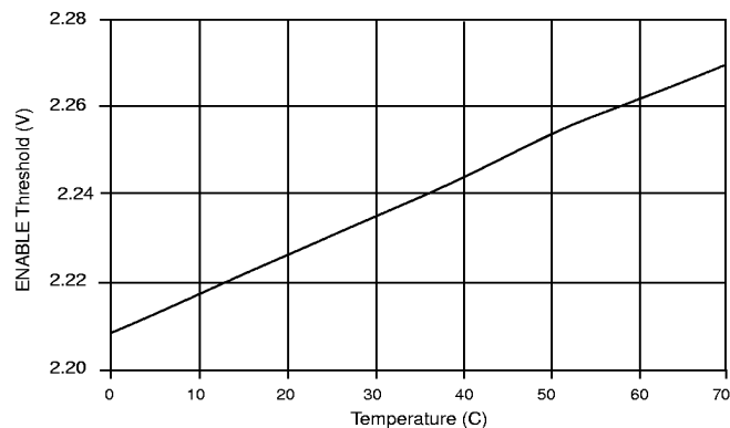
Figure 38: ENABLE Threshold vs Temperature.
