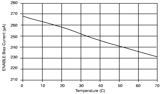
Figure 36: ENABLE Bias Current vs Temperature.
