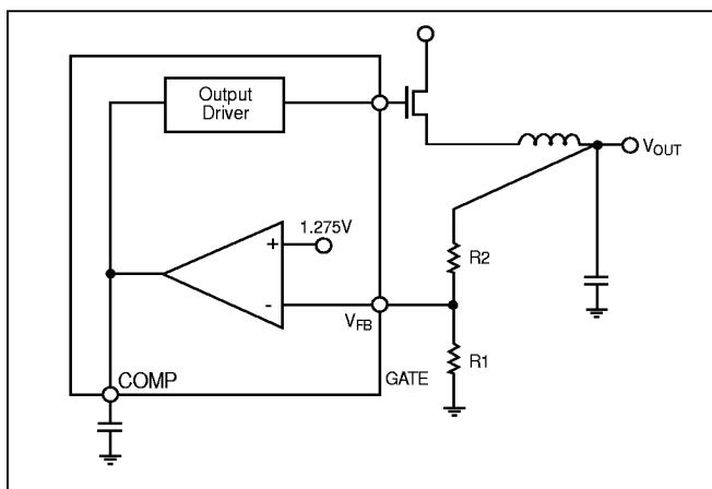
Figure 3: Feedback resistor divider.
