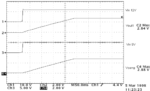
Figure 5: Measured performance of the CS-5127 at start up. C_{\text{COMP}} = 100\mu\text{F} , I_{\text{COMP(SOURCE)}} = 1.3\text{mA} , V_{\text{FFB}} = 2.8\text{V} , T_{\text{SOFTSTART}} = 0.22\text{s} .
