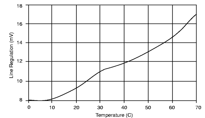
Figure 20: Line Regulation vs Temperature 9V to 25V.
