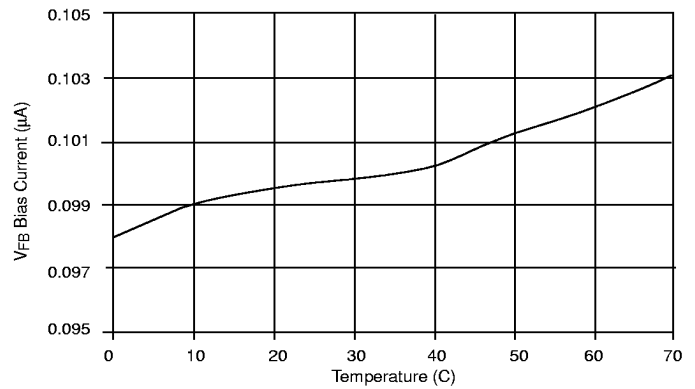
Figure 31: V_{\text{FB}} Bias Current vs Temperature.
