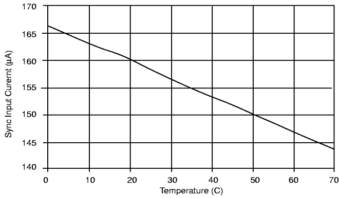
Figure 24: SYNC Input Current vs Temperature ( V_{\text{SYNC}} = 2.4\text{V} ).
