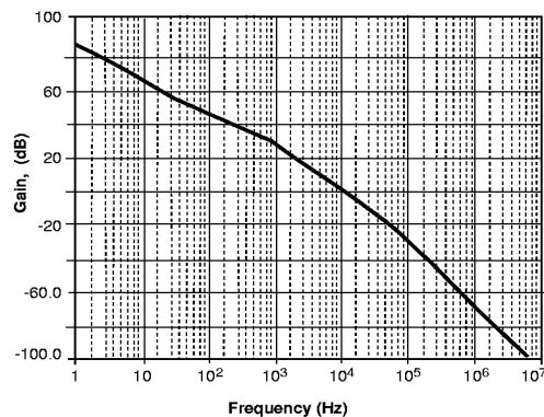
Figure 9: Bode plot of gain response for compensated voltage mode system
