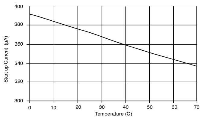
Figure 46: Start-up Current vs Temperature.
