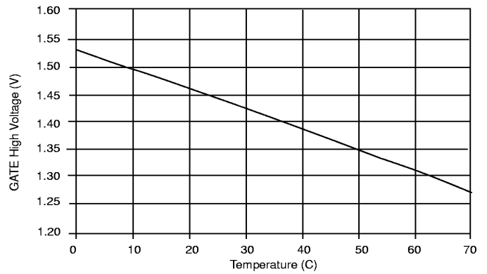
Figure 43: GATE High Voltage (20mA) vs Temperature
