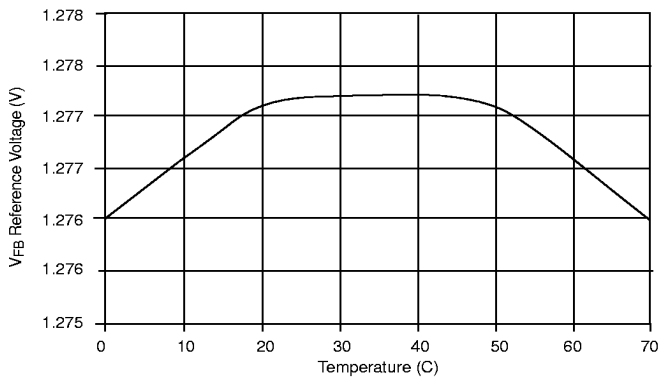
Figure 28: V_{\text{FB}} Reference Voltage vs Temperature.
