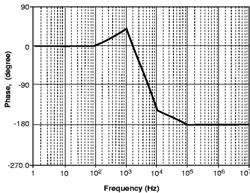
Figure 8: Bode plot of phase response for V_{OUT}/V_{CONTROL}
