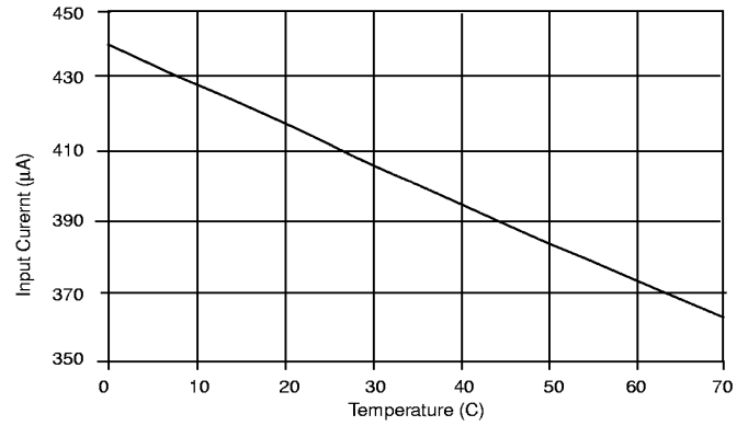
Figure 27: SYNC Input Current vs Temperature ( V_{\text{SYNC}} = 5\text{V} ).
