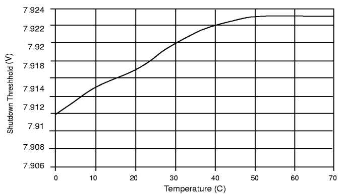
Figure 45: V_{IN} Shutdown Threshold vs Temperature.
