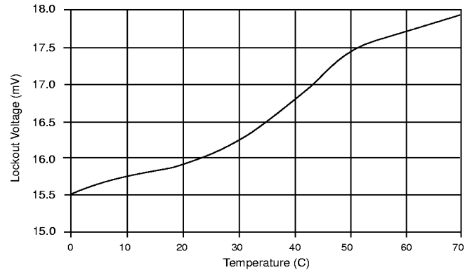
Figure 44: GATE Low Voltage (Lockout) vs Temperature.
