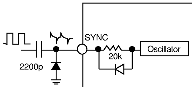
Figure : Capacitive coupling of the SYNC signal. The external diode is used to clamp the IC substrate diode if I_{SYNC} is greater than 5mA during the negative portion of the input waveform.
