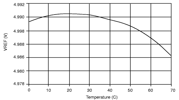
Figure19: V REF vs Temperature, 10mA Load.
