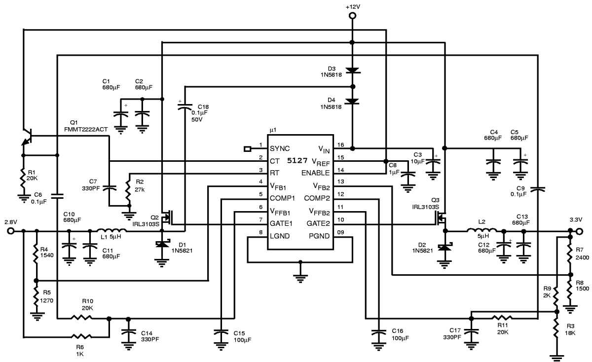
Figure 15: 2.8V @ 7A and 3.3V @ 7A 12V only application circuit.
