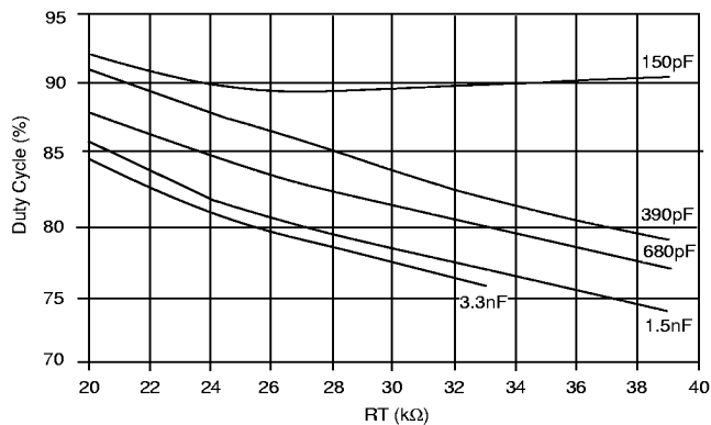
Figure 25: Oscillator Duty Cycle vs C T , R T (V IN = 12V, T = 25°C).
