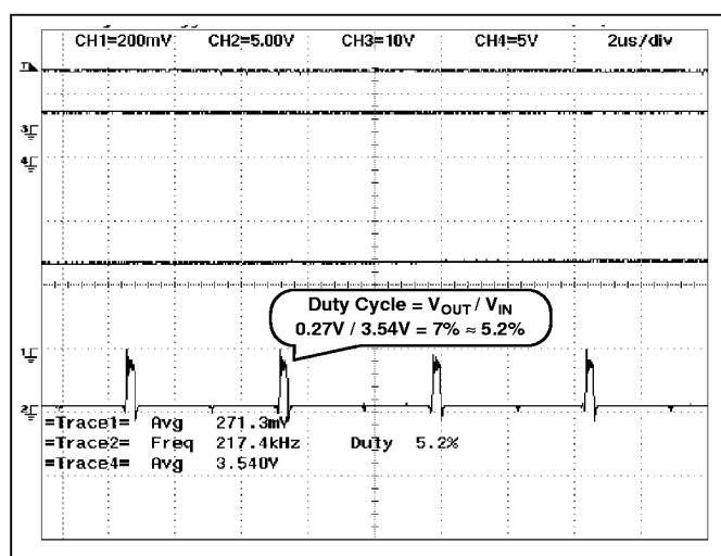
Figure 4: Pulse-by-Pulse Regulation during Soft Start (2μs/div).
