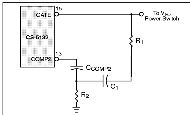
Figure 7: Slope compensation for the non-synchronous regulator section ( V_{I/O} ).
