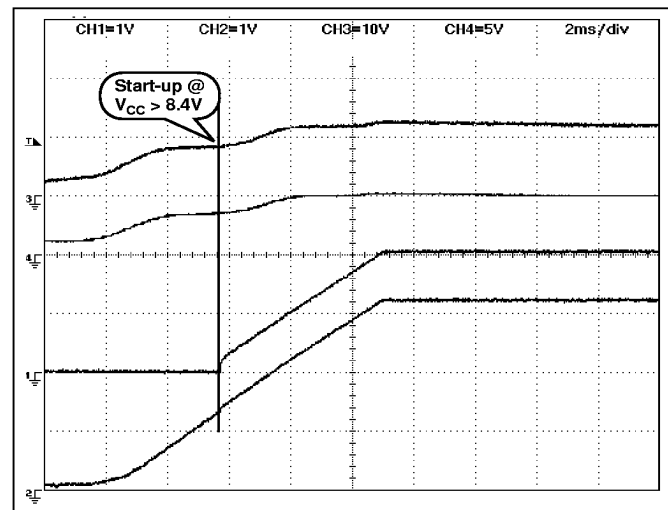
Figure 2: Normal Start-up (2ms/div).
