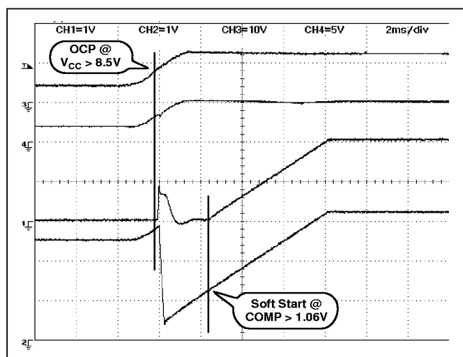
Figure 5: Start-up with COMP pre-charged to 2V (2ms/div).
