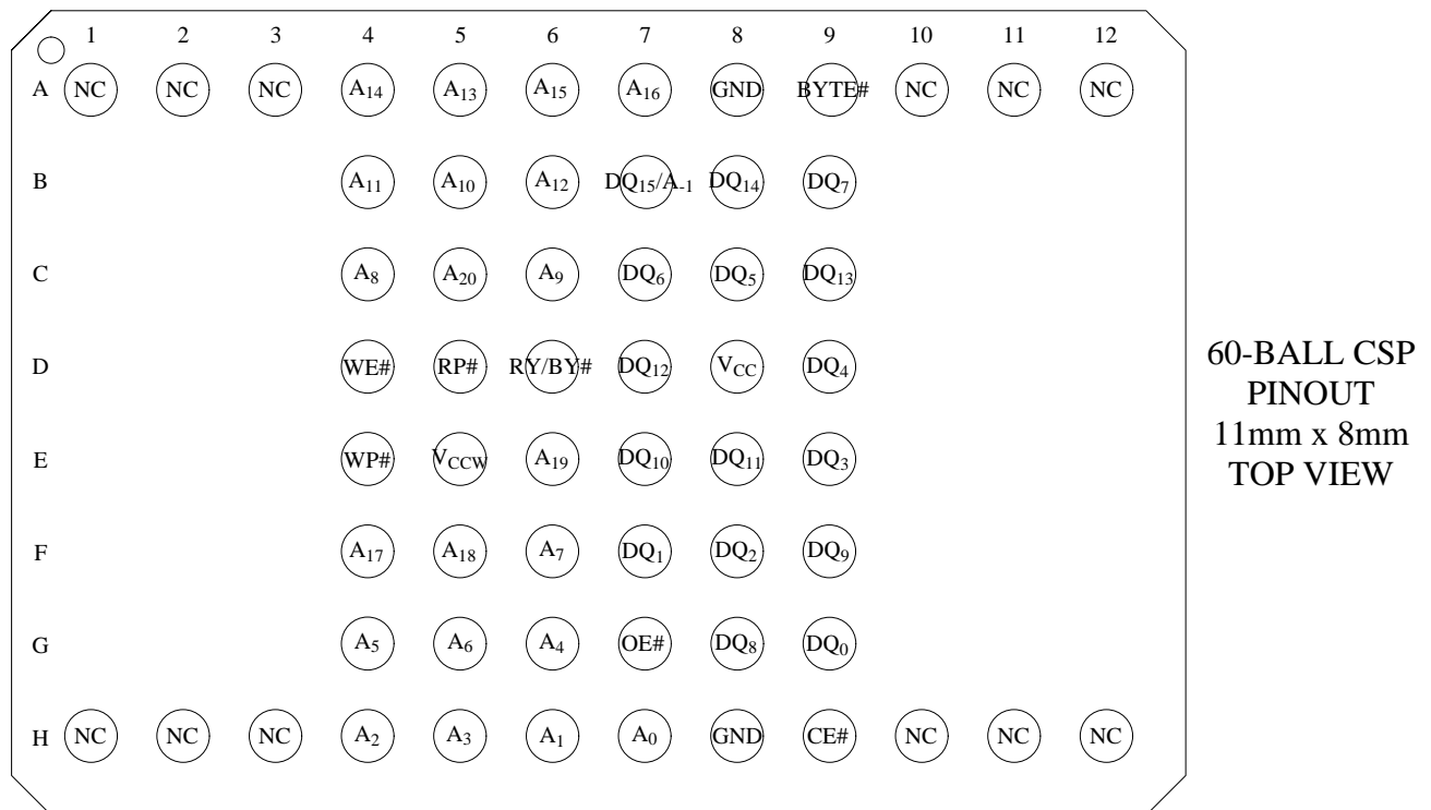
Figure 2. CSP 60-Ball Pinout
