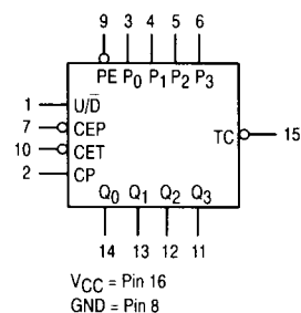
LOGIC SYMBOL
