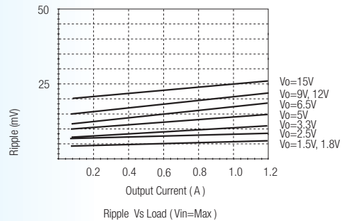
Ripple Vs Load (Vin=Max)
