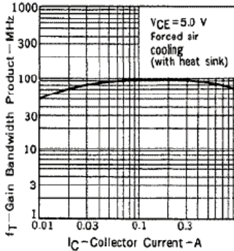
GAIN BANDWIDTH PRODUCT vs. COLLECTOR CURRENT
