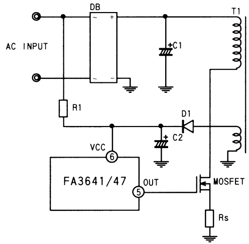
Fig. 19 Startup circuit (1)
