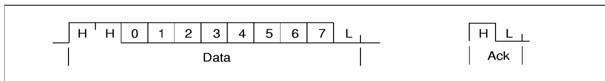
Figure 8.1 IMS T805E link data and acknowledge packets
