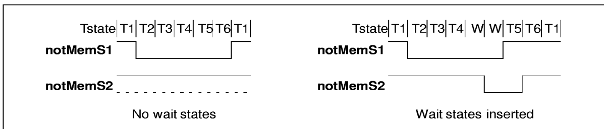
Figure 6.6 IMS T805E effect of wait states on strobes
