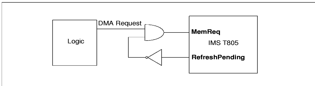
Figure 6.10 IMS T805E refresh with DMA
