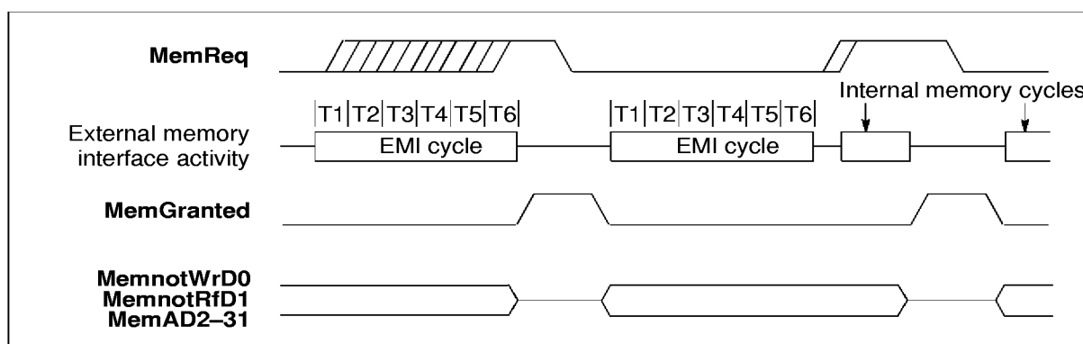
Figure 6.16 IMS T805E operation of MemReq , MemGranted with external, internal memory cycles
