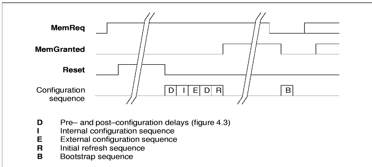
Figure 6.14 IMS T805E DMA sequence at reset
