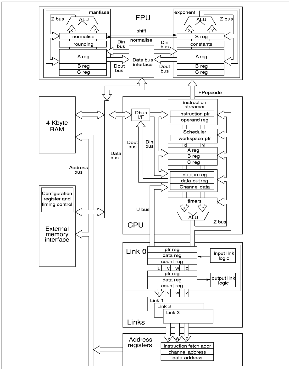
Figure 1.2 IMS T805E internal datapaths
