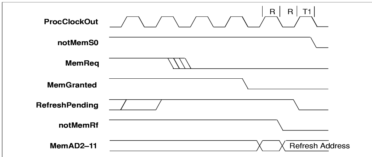
Figure 6.12 IMS T805E refresh pending timing diagram
