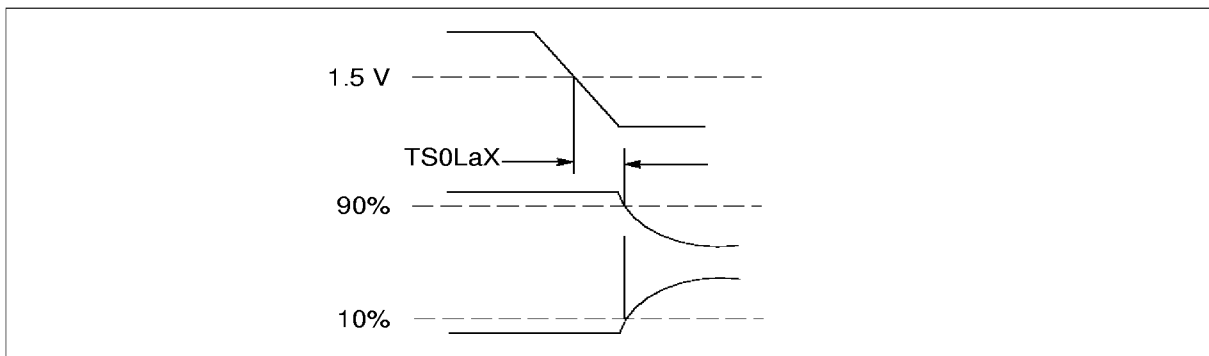
Figure 9.4 IMS T805E tristate timing relative to notMemS0
