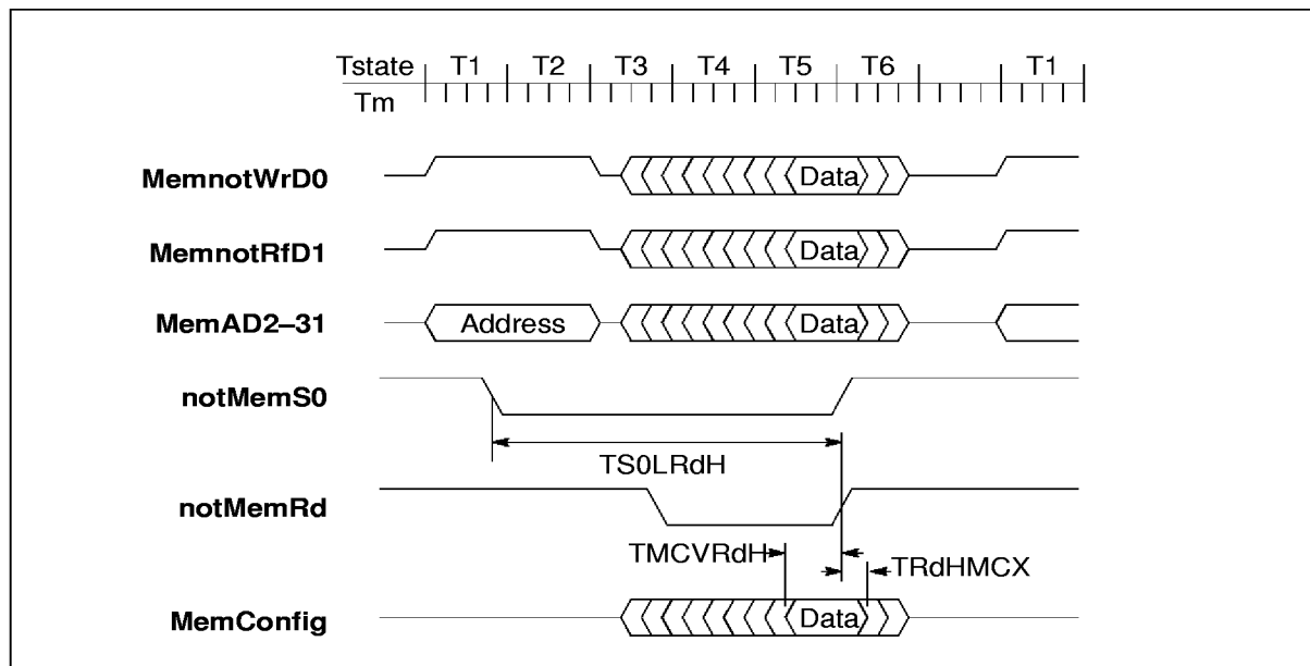
Figure 6.21 IMS T805E external configuration read cycle timing
