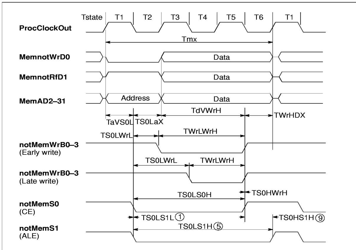
Figure 6.8 IMS T805E external write cycle
