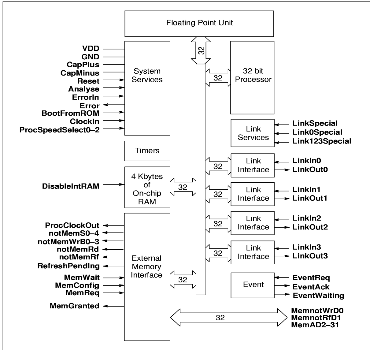
Figure 1.1 IMS T805E block diagram
