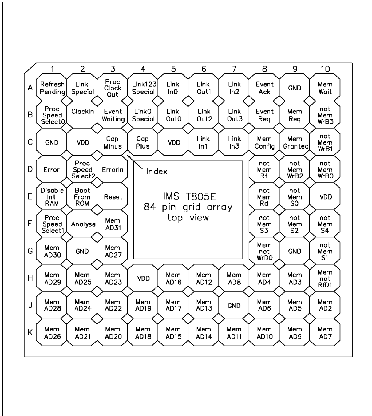
Figure 10.1 IMS T805E 84-pin grid array package pinout
