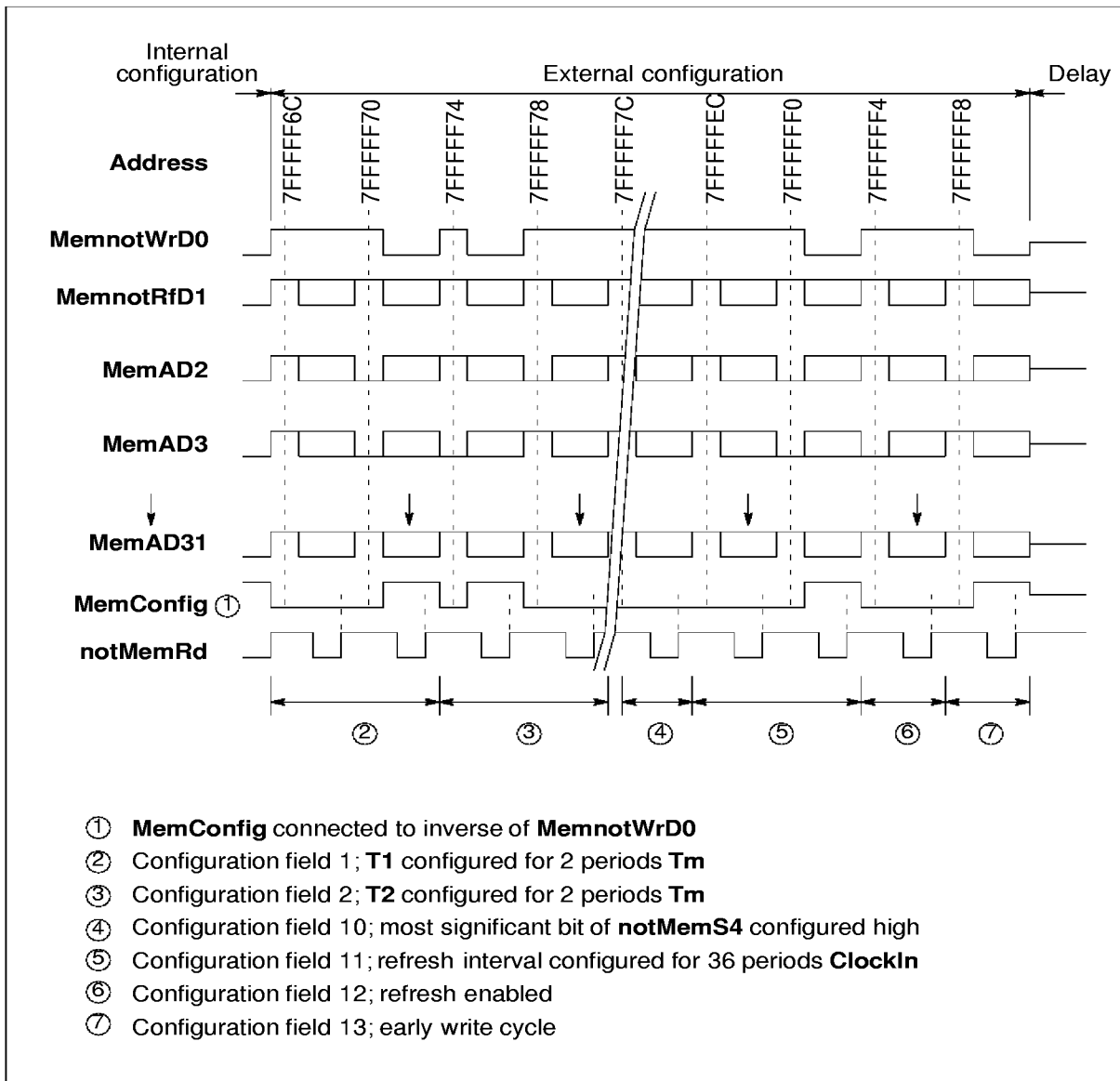
Figure 6.20 IMS T805E external configuration scan
