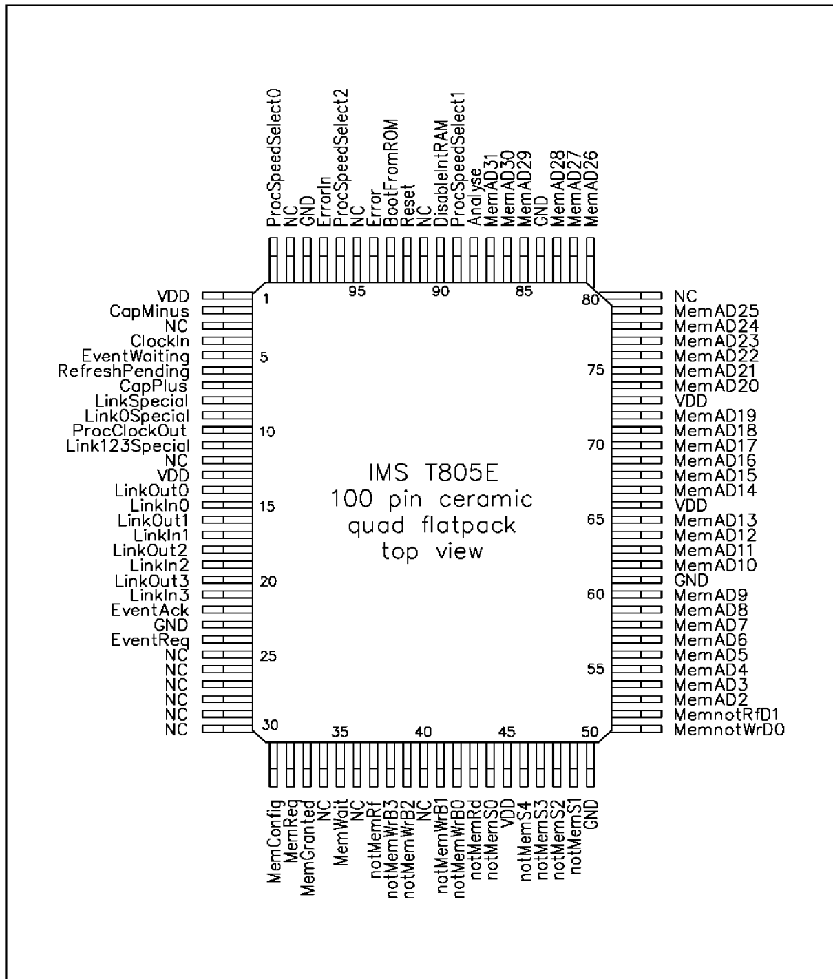
Figure 10.3 IMS T805E 100-pin cavity-down ceramic quad flat pack (CQFP) package pinout
