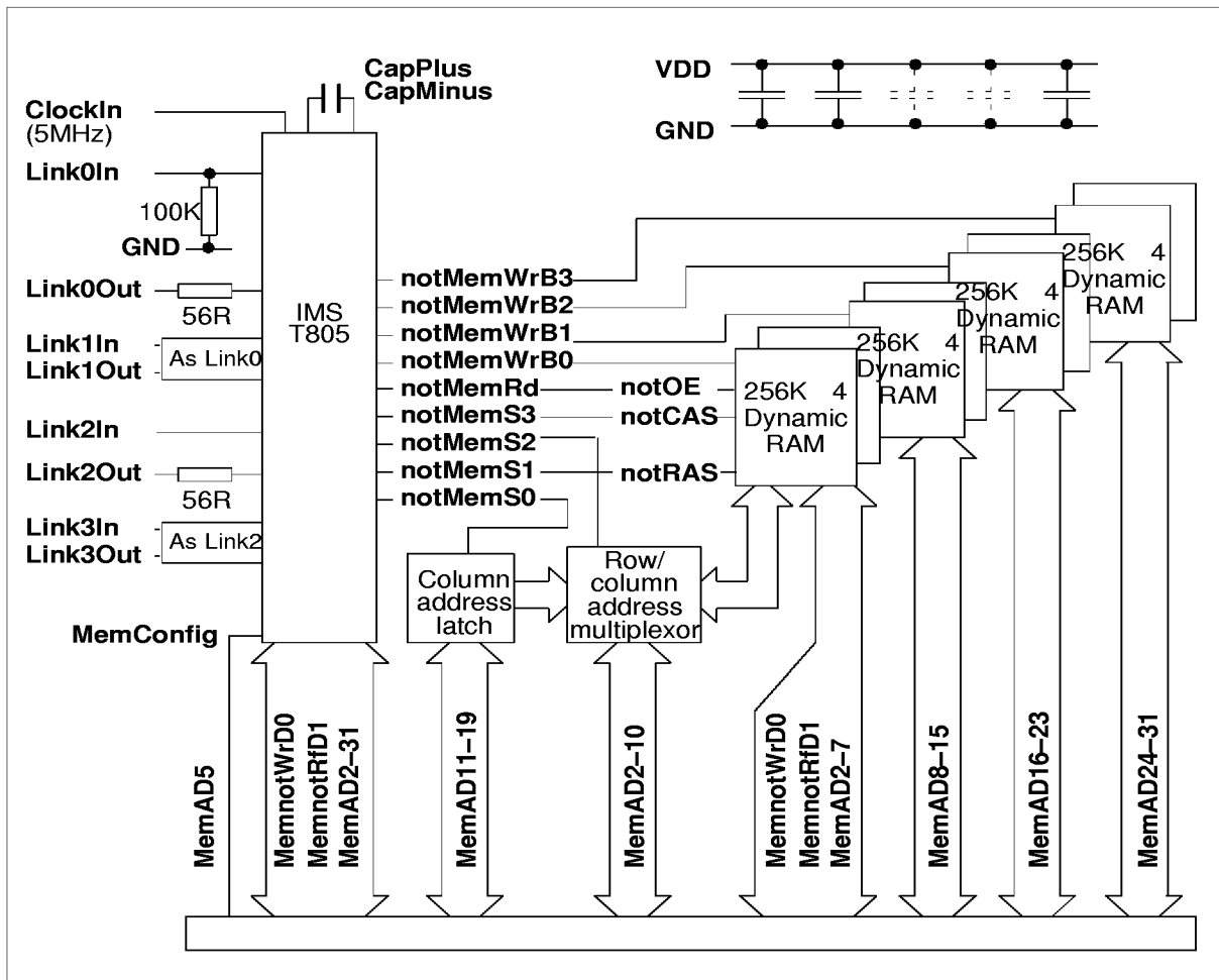
Figure 6.2 IMS T805E application
