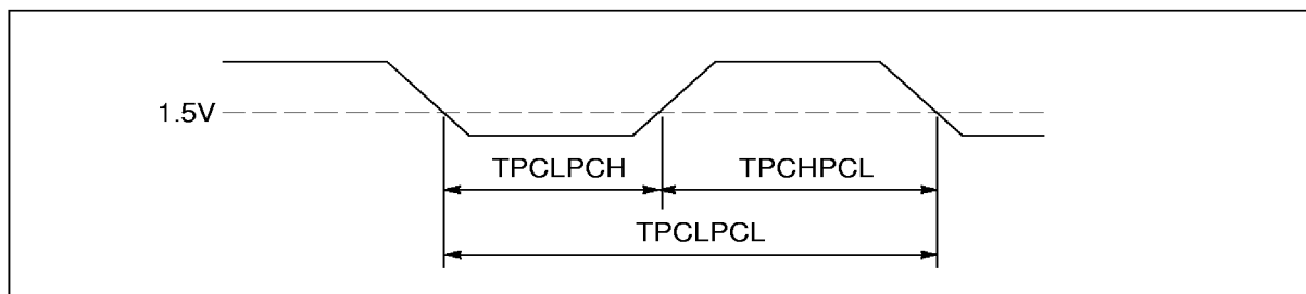
Figure 6.3 IMS T805E ProcClockOut timing
