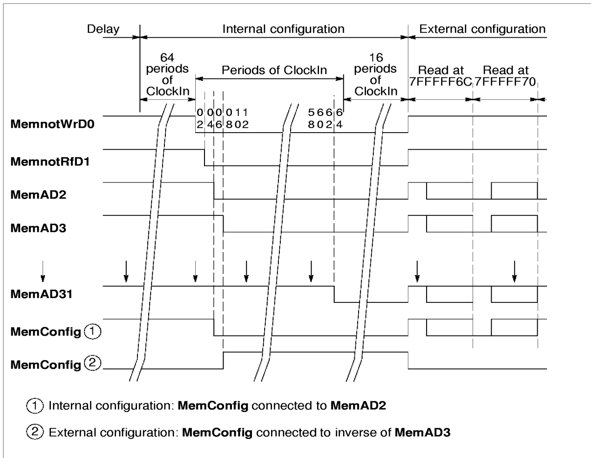
Figure 6.18 IMS T805E internal configuration scan
