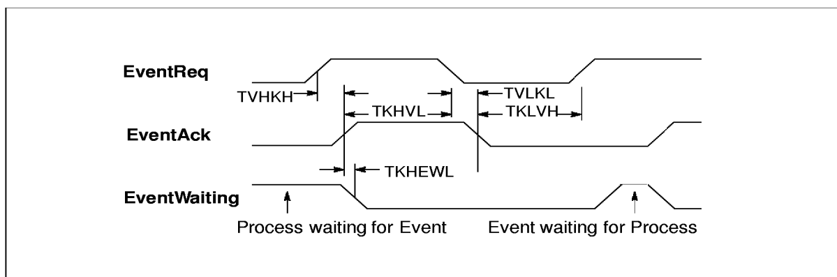
Figure 7.1 IMS T805E event timing
