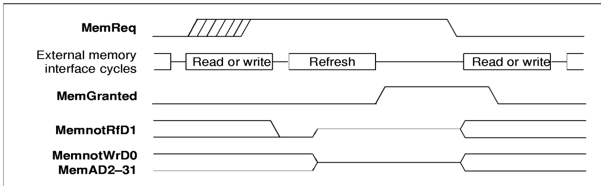
Figure 6.15 IMS T805E operation of MemReq , MemGranted with external, refresh memory cycles
