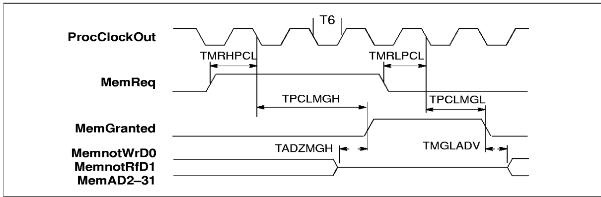
Figure 6.13 IMS T805E memory request timing
