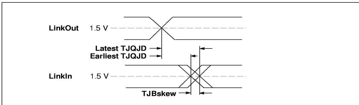
Figure 8.3 IMS T805E buffered link timing
