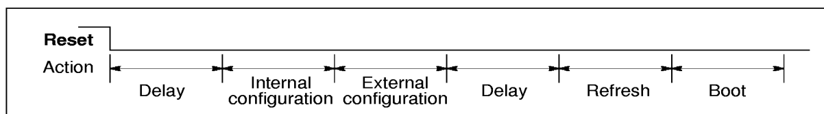
Figure 4.3 IMS T805E post-reset sequence
