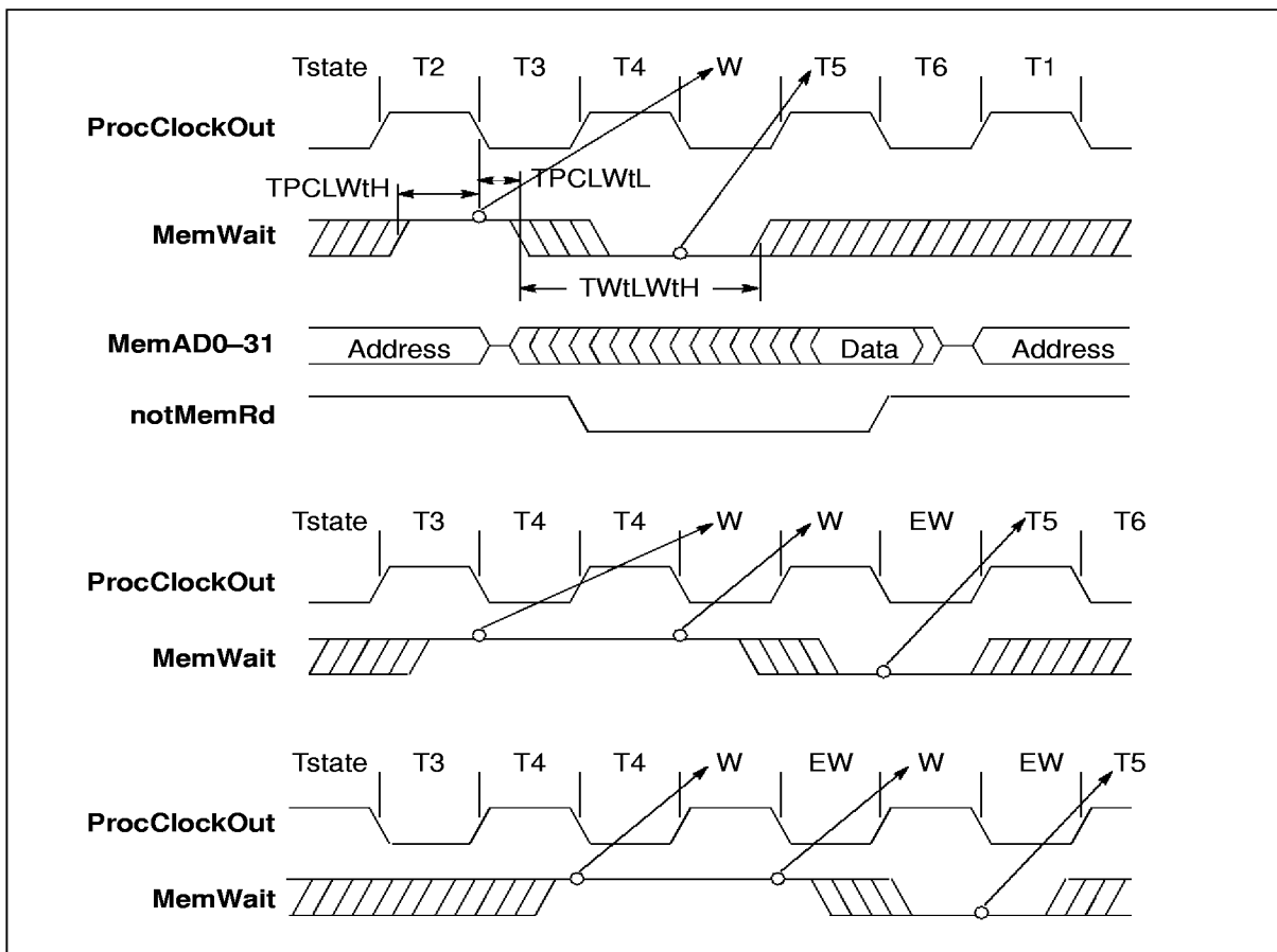
Figure 6.9 IMS T805E memory wait timing
