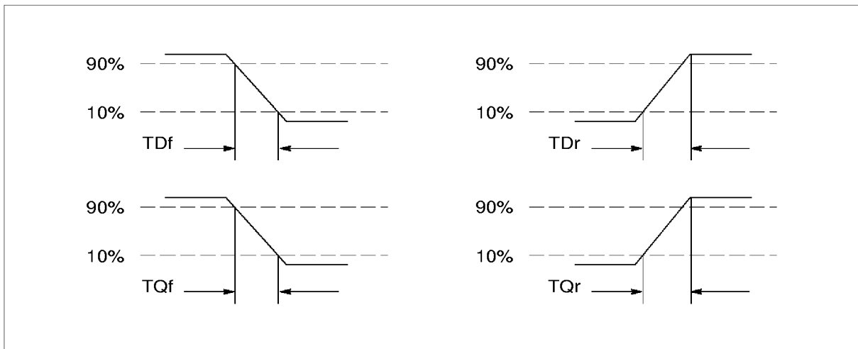
Figure 9.3 IMS T805E input and output edge timing
