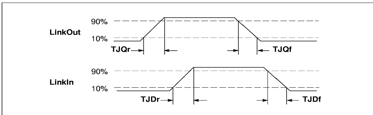
Figure 8.2 IMS T805E link timing
