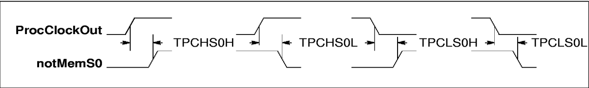
Figure 6.7 IMS T805E skew of notMemS0 to ProcClockOut
