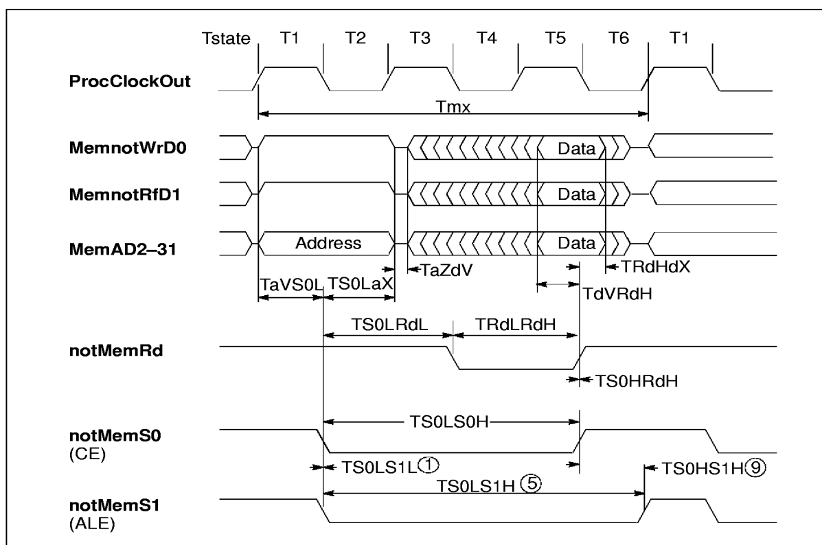
Figure 6.4 IMS T805E external read cycle: static memory
