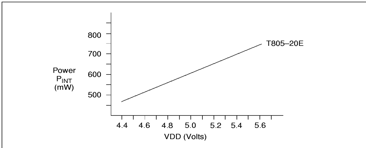
Figure 9.6 IMS T805E internal power dissipation vs VDD
