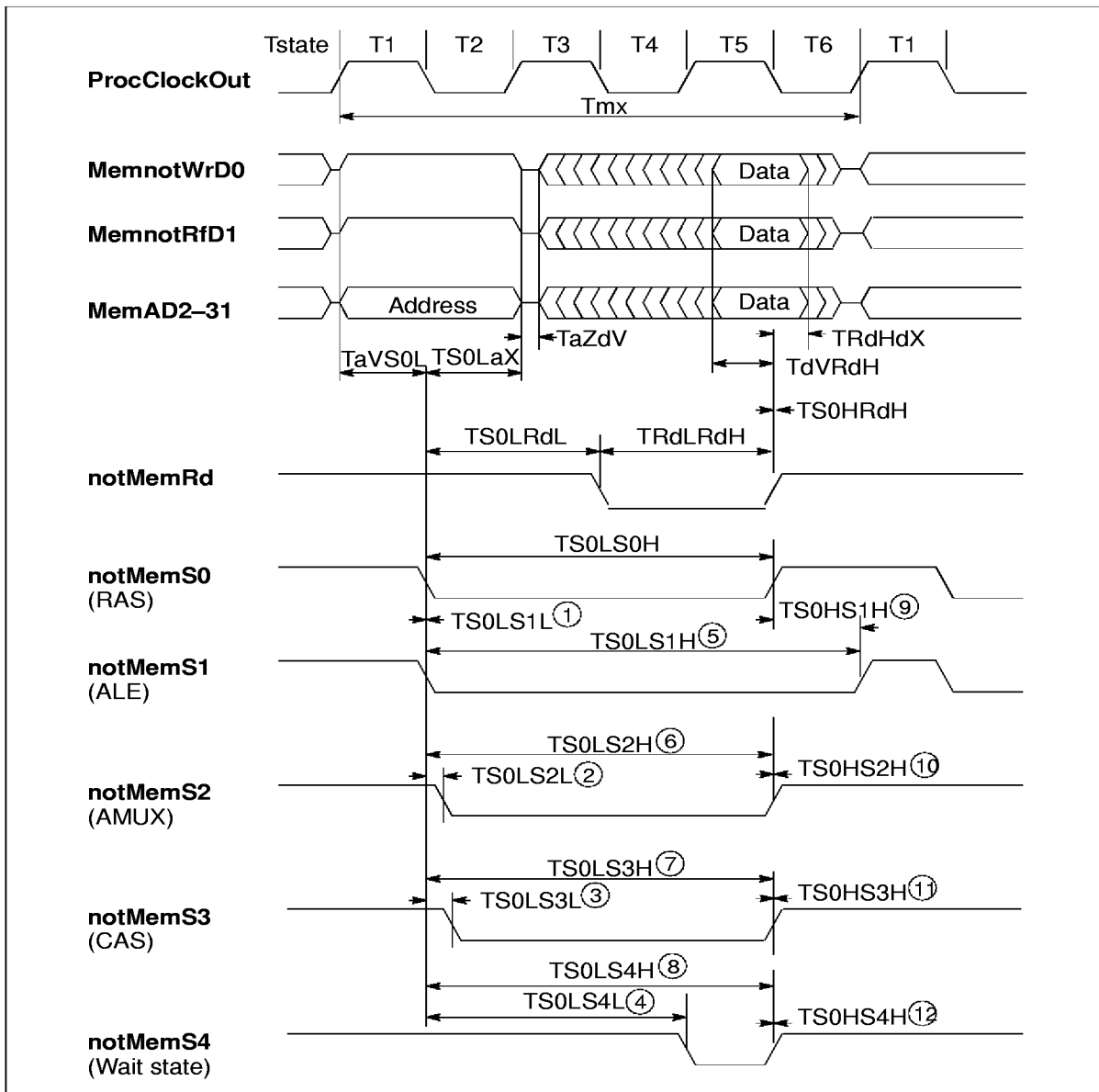
Figure 6.5 IMS T805E external read cycle: dynamic memory
