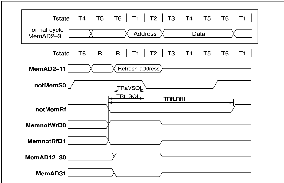
Figure 6.11 IMS T805E refresh cycle timing
