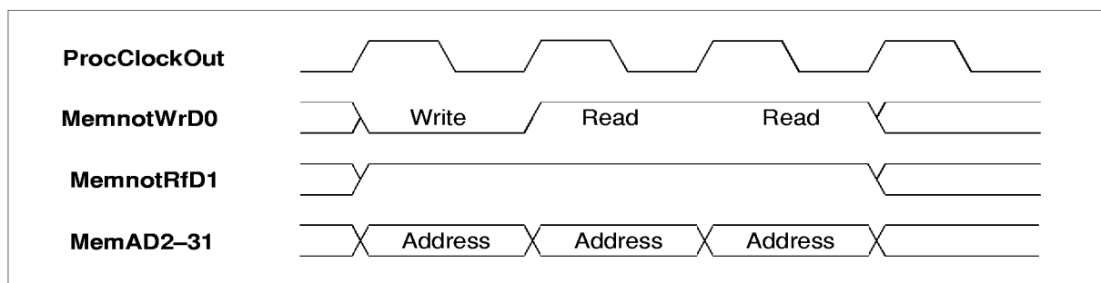
Figure 6.1 IMS T805E bus activity for internal memory cycle
