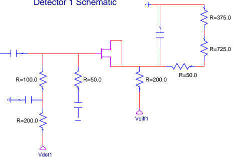
Detector 1 Schematic
