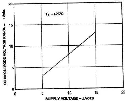
Figure 1. Input Common-Mode Voltage Range vs. Supply
