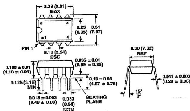
8-Lead Cerdip (Q) Package
