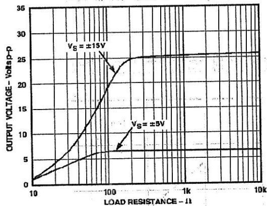
Figure 2. Output Voltage Swing vs. Resistive Load
