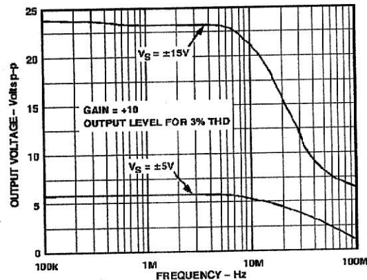
Figure 16. Large Signal Frequency Response
