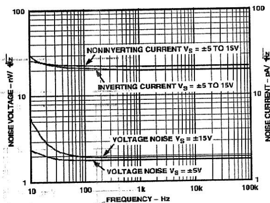
Figure 11. Input Noise vs. Frequency
