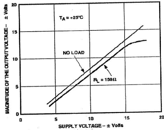
Figure 4. Output Voltage Swing vs. Supply
