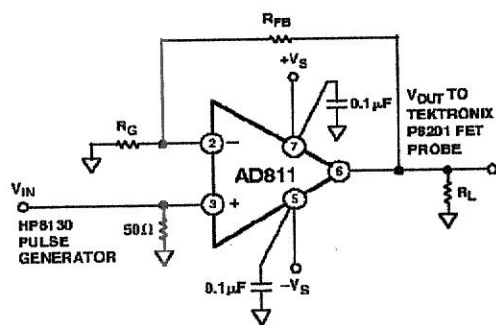
Figure 19. Noninverting Amplifier Connection
