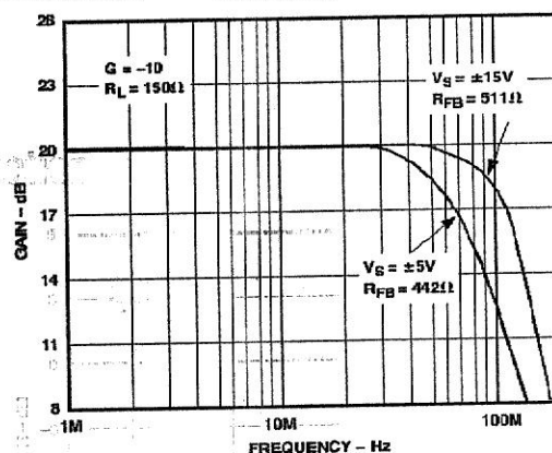
Figure 29. Closed-Loop Gain vs. Frequency, Gain = -10
