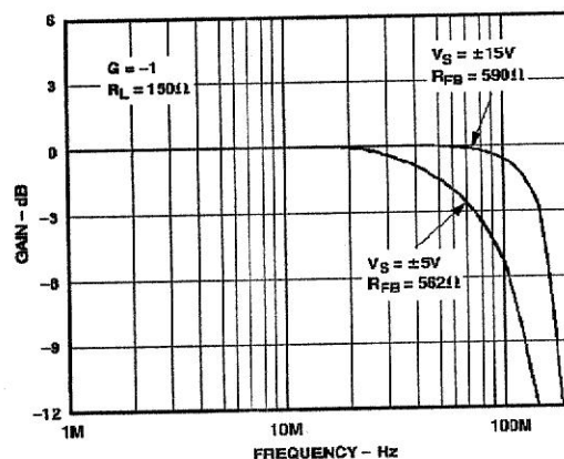
Figure 28. Closed-Loop Gain vs. Frequency, Gain = -1
