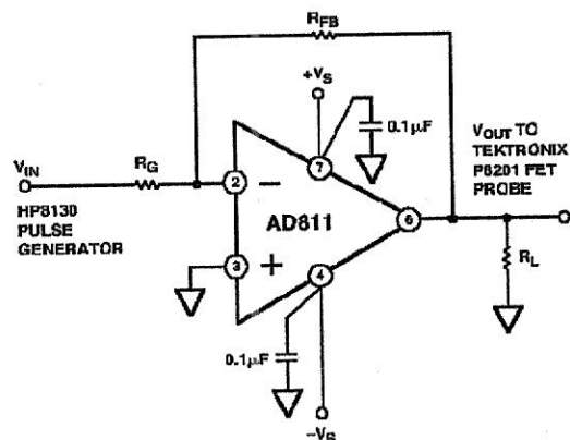
Figure 25. Inverting Amplifier Connection
