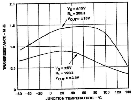
Figure 10. Transresistance vs. Junction Temperature
