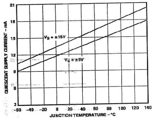
Figure 5. Quiescent Supply Current vs. Junction Temperature
