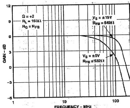
Figure 36. Closed-Loop Gain vs. Frequency, Gain = +2
