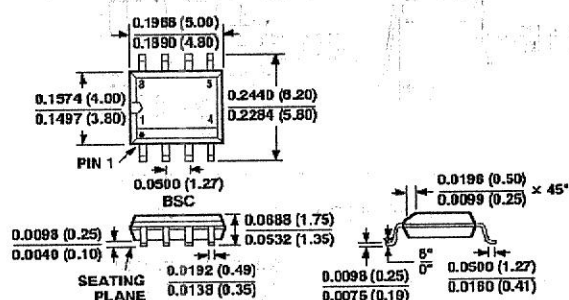
8-Lead SOIC (SO-8) Package
