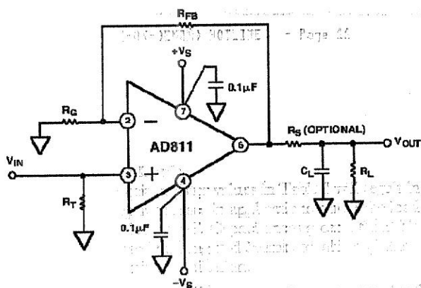
Figure 31. Recommended Connection for Driving a Large Capacitive Load
