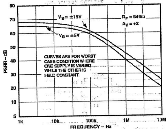
Figure 14. Power Supply Rejection vs. Frequency
