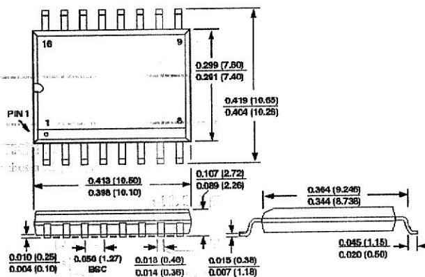
16-Lead SOIC (R-16) Package
