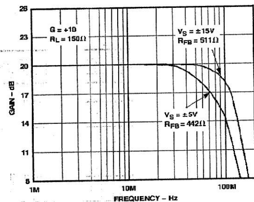
Figure 23. Closed-Loop Gain vs. Frequency, Gain = +10
