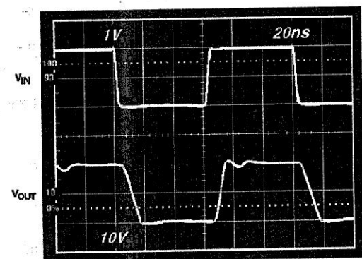
Figure 24. Large Signal Pulse Response, Gain = +10
