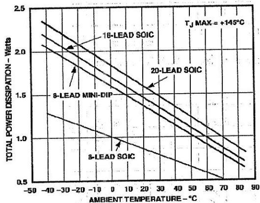
Figure 15. Maximum Power Dissipation vs. Temperature for Plastic Packages
