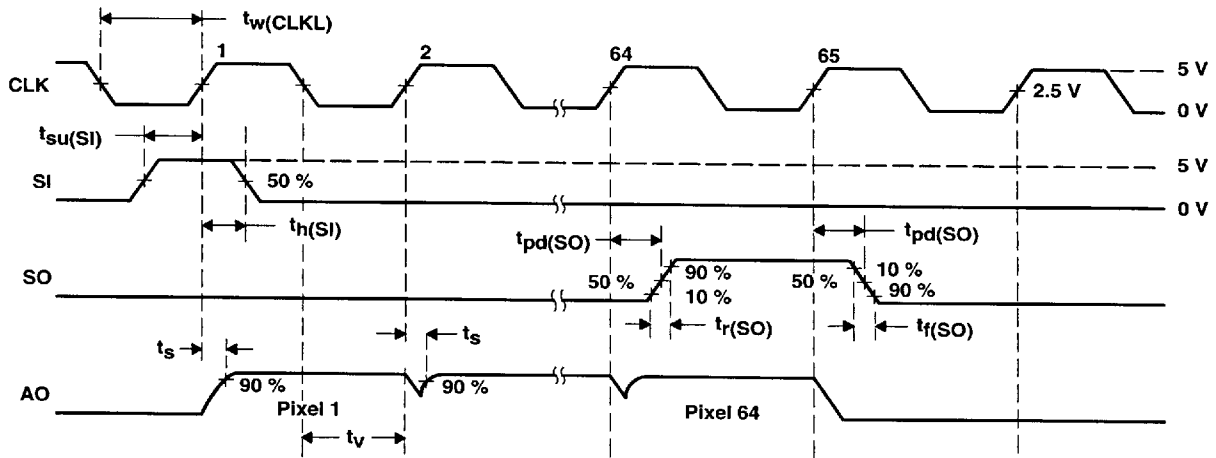
Figure 2. Test Circuit and Operational Waveforms
