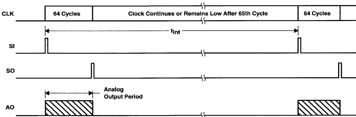
Figure 1. Timing Waveforms
