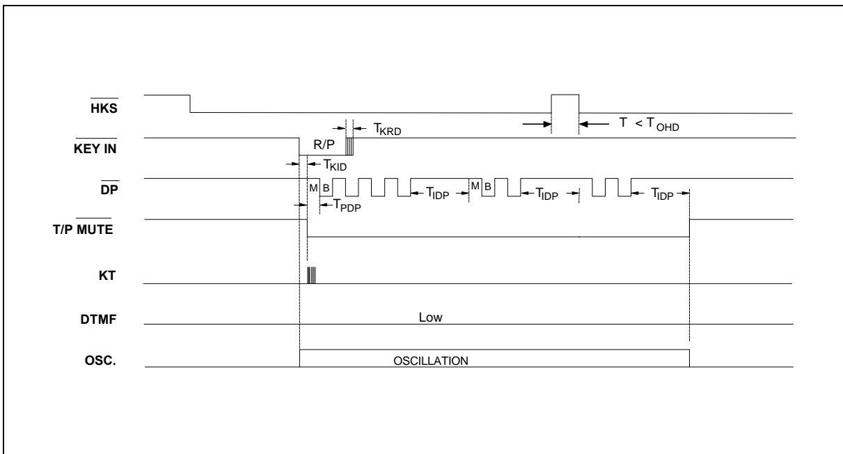
Figure 1(b) Pulse Mode Auto Dialing Timing Diagram
