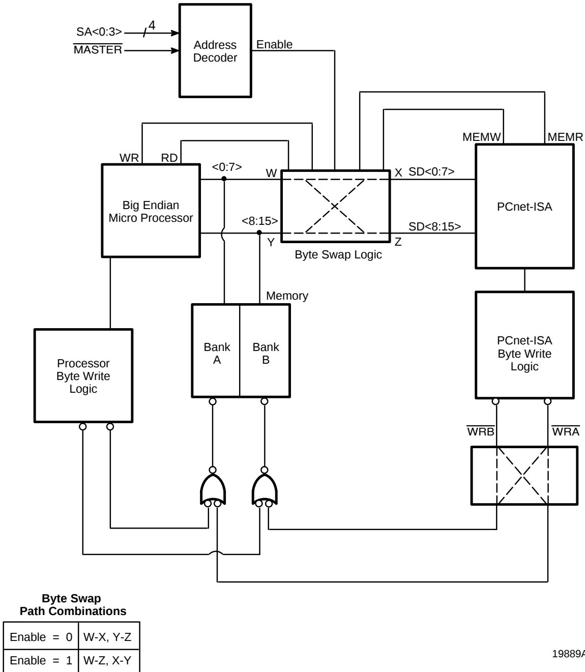
Figure 20. Logical Block Diagram for Byte Swap
