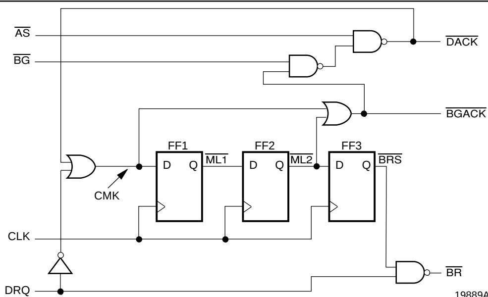
Figure 14. Bus Master Exchange Circuit
