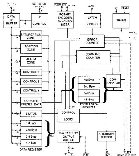
BLOCK DIAGRAM
