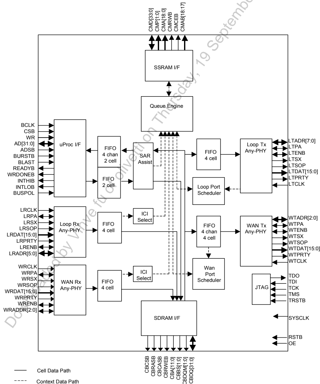
Figure 2 - S/UNI-APEX-1K800 Block Diagram With Datapath
