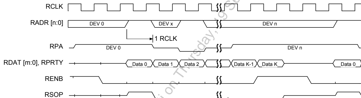
Figure 45 - UTOPIA L2 Receive Master (Loop & WAN)
