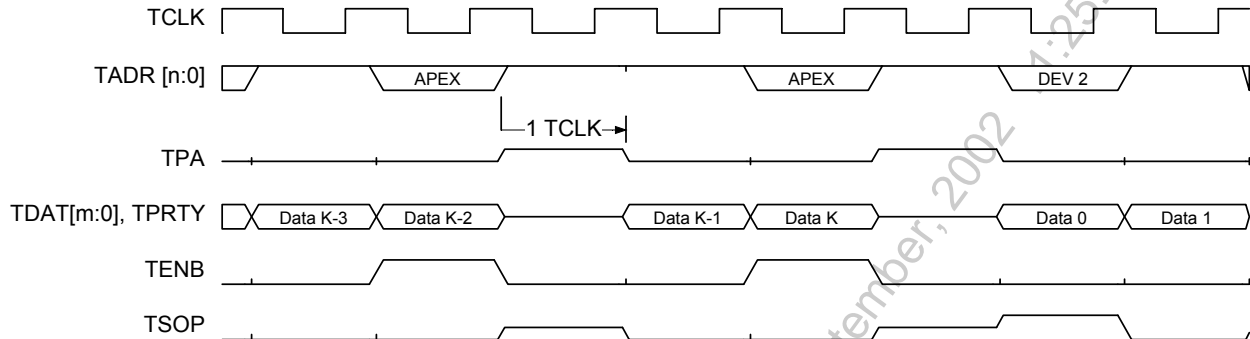
Figure 47 - UTOPIA L2 Receive Slave (Loop & WAN)
