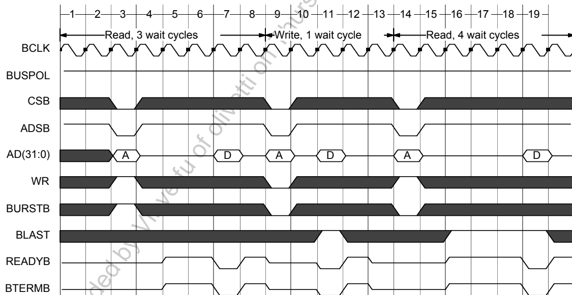
Figure 34 - Single Word Read and Write to Non-burstable Address Space
