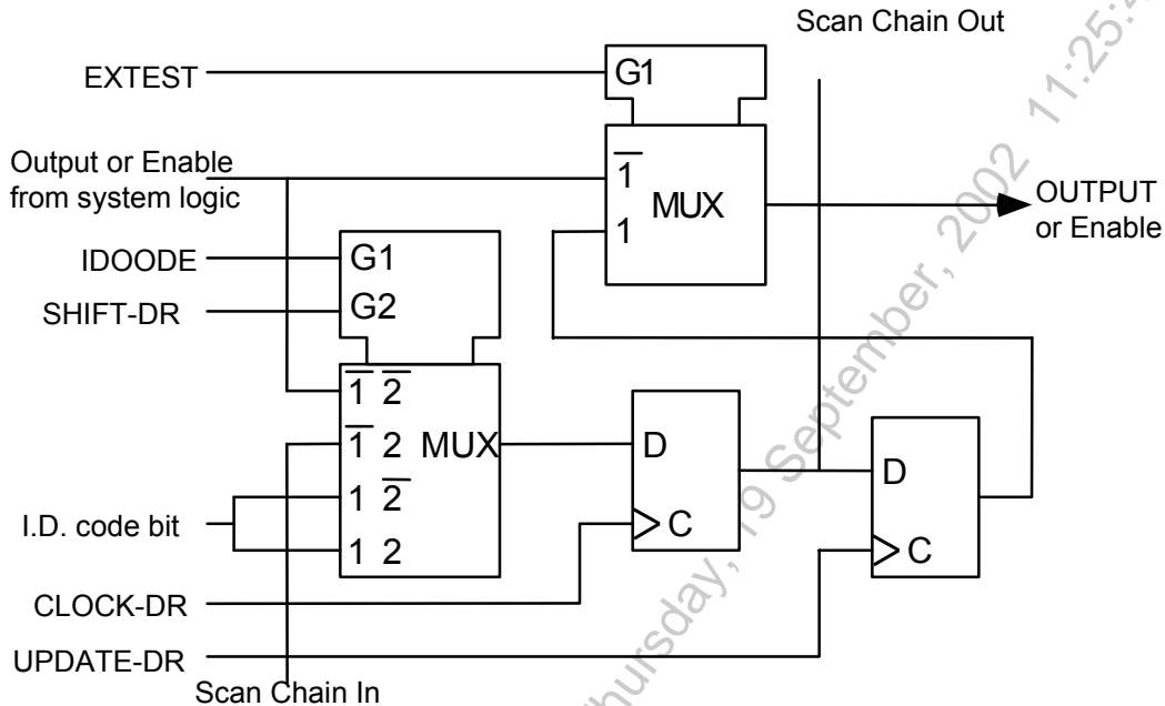
Figure 31 - Output Cell (OUT_CELL)
