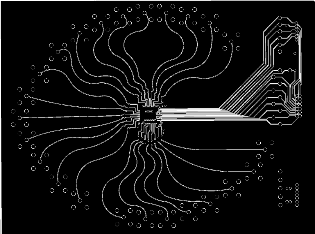
Figure 49. Board Layout (Signal Layer)
