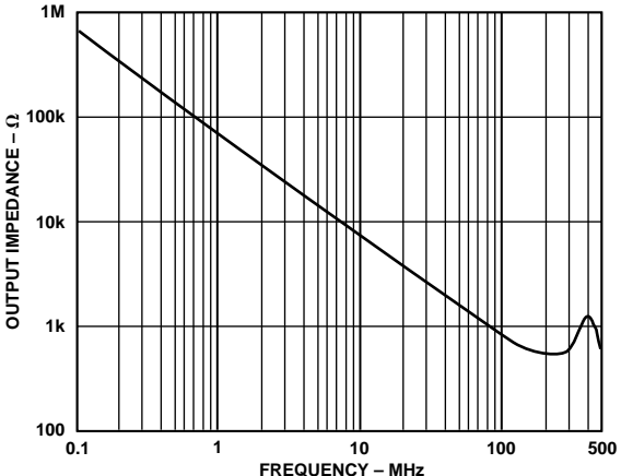
Figure 20. AD8108 Output Impedance, Disabled
