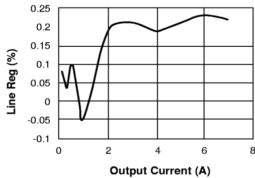
Line Regulation vs. Output Load ( F_{OSC} = 1 \text{ MHz} )
