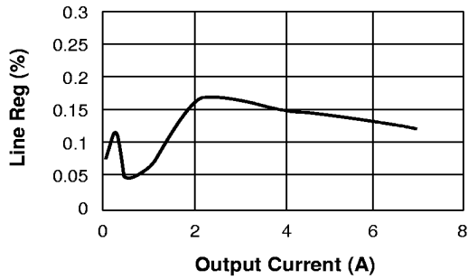
Line Regulation vs. Output Load ( F_{OSC} = 650 \text{ KHz} )
