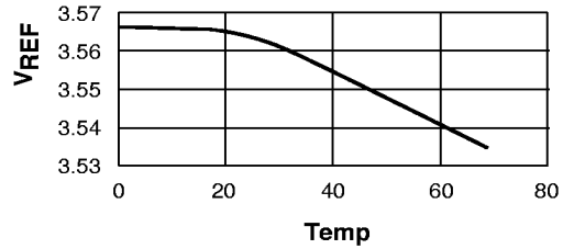
Reference Tempco
