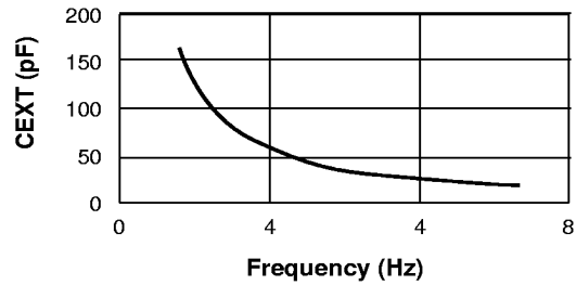
CEXT vs. Oscillator Frequency
