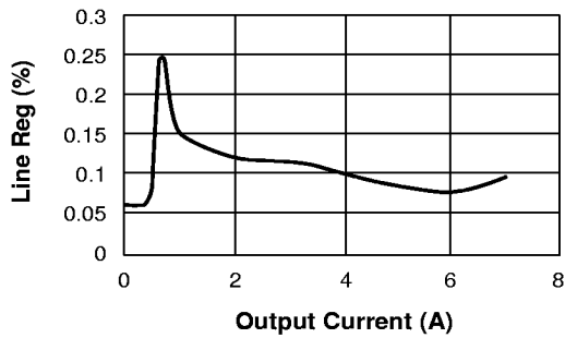
Line Regulation vs. Output Load ( F_{OSC} = 400 \text{ KHz} )
