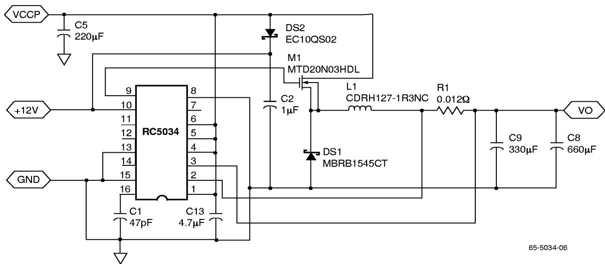
Figure 2. Non-Synchronous 7A Circuit
