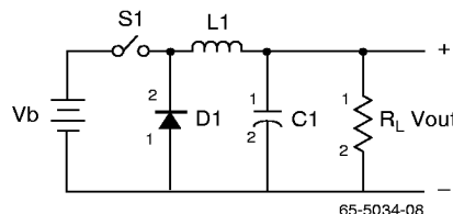
Figure 4. Simple Buck DC-DC Converter
