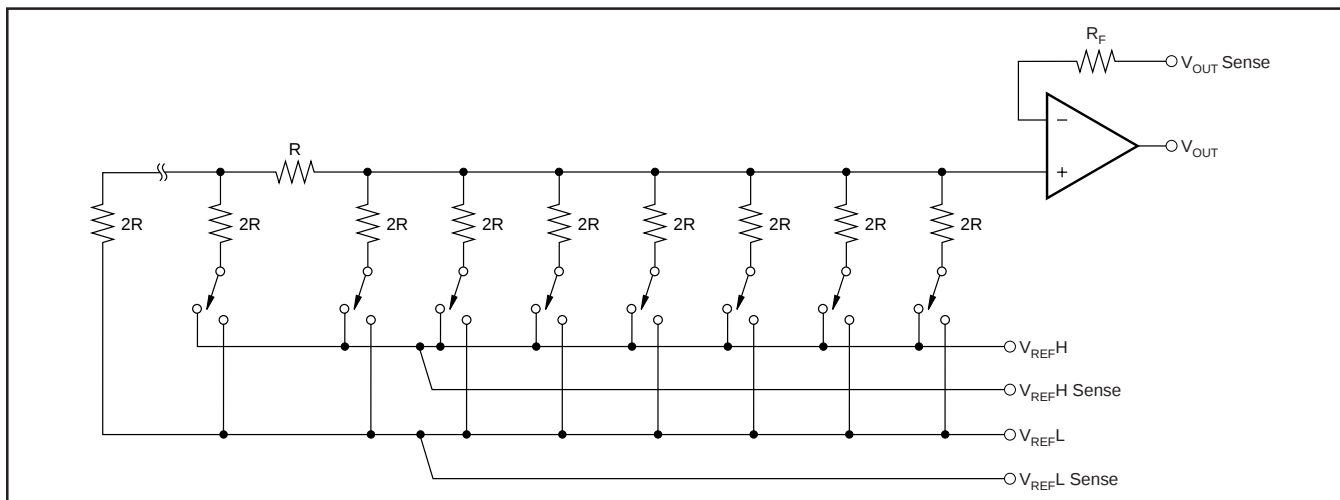
FIGURE 1. DAC7734 Architecture.
