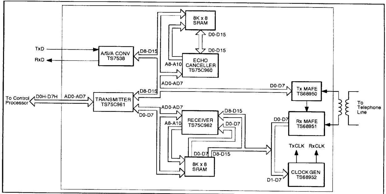
Figure 5 : Hardware Architecture
