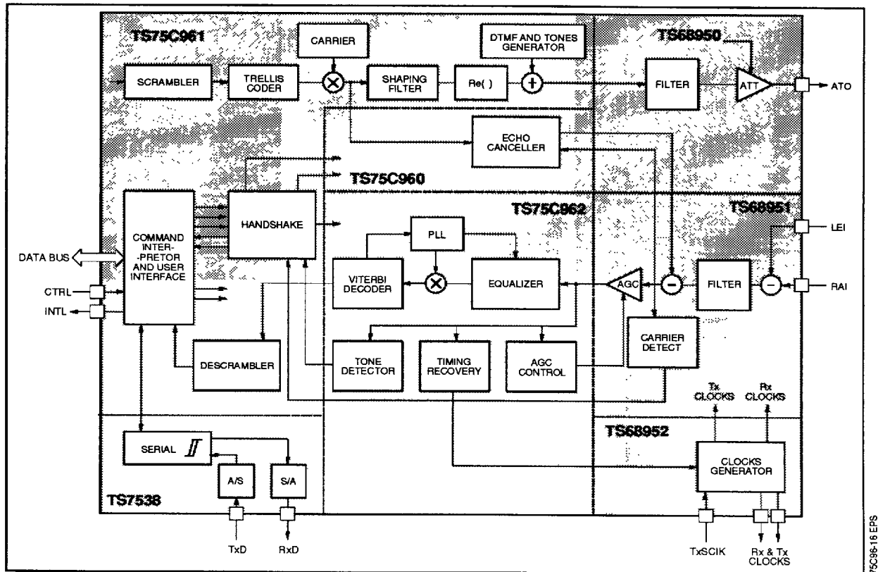
Figure 6 : Functional Block Diagram (V.32 Operation)
