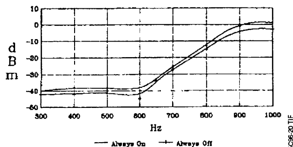
Figure 10 : Band 1 Tone Detector
