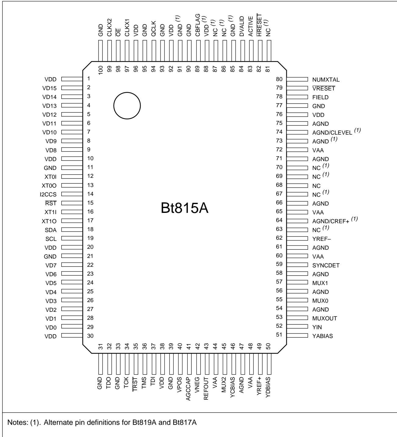
Figure 4. Bt815A Pinout
