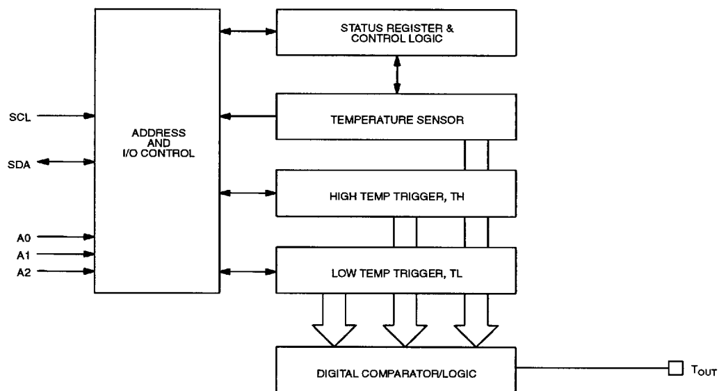
DS1622 FUNCTIONAL BLOCK DIAGRAM Figure 1
