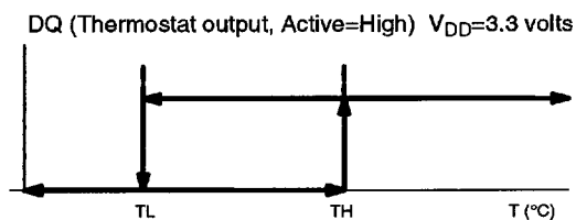
THERMOSTAT OUTPUT OPERATION Figure 3
