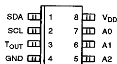
DS1622S 8-PIN SOIC (150 MIL)
