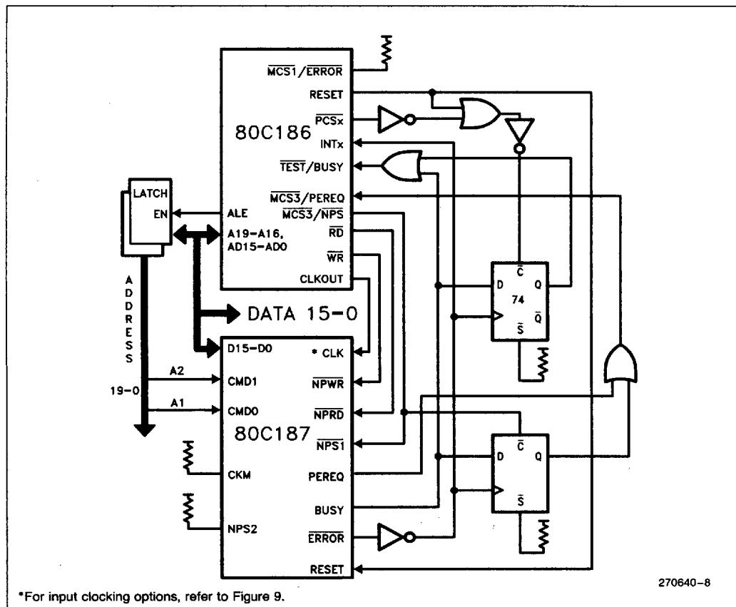
Figure 10. System Configuration for 8087-Compatible Exception Trapping
