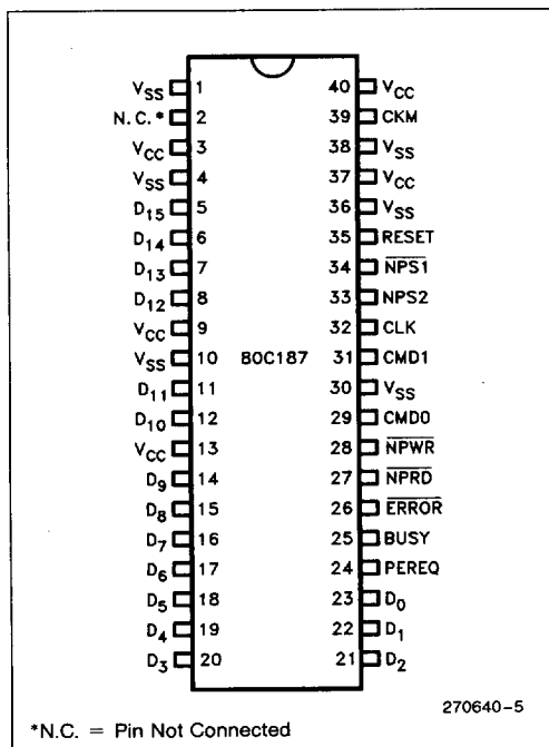
Figure 7. Cerdip Pin Configuration
