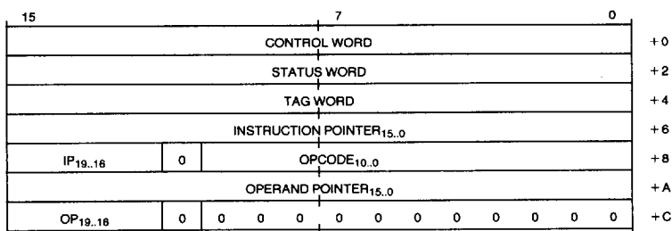
Figure 6. Instruction and Data Pointer Image in Memory
