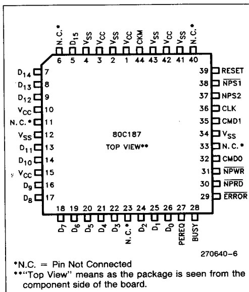
Figure 8. PLCC Pin Configuration
