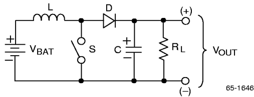
Figure 6. Simple Set-Up Converter
