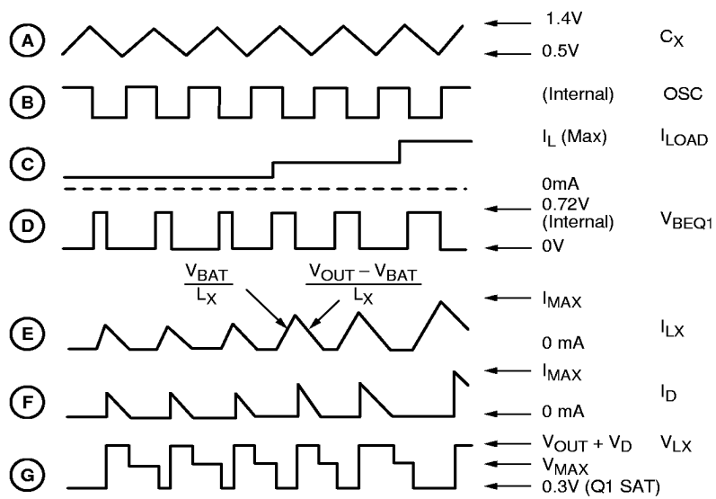
Figure 8. Step-Up Regulator Waveforms
