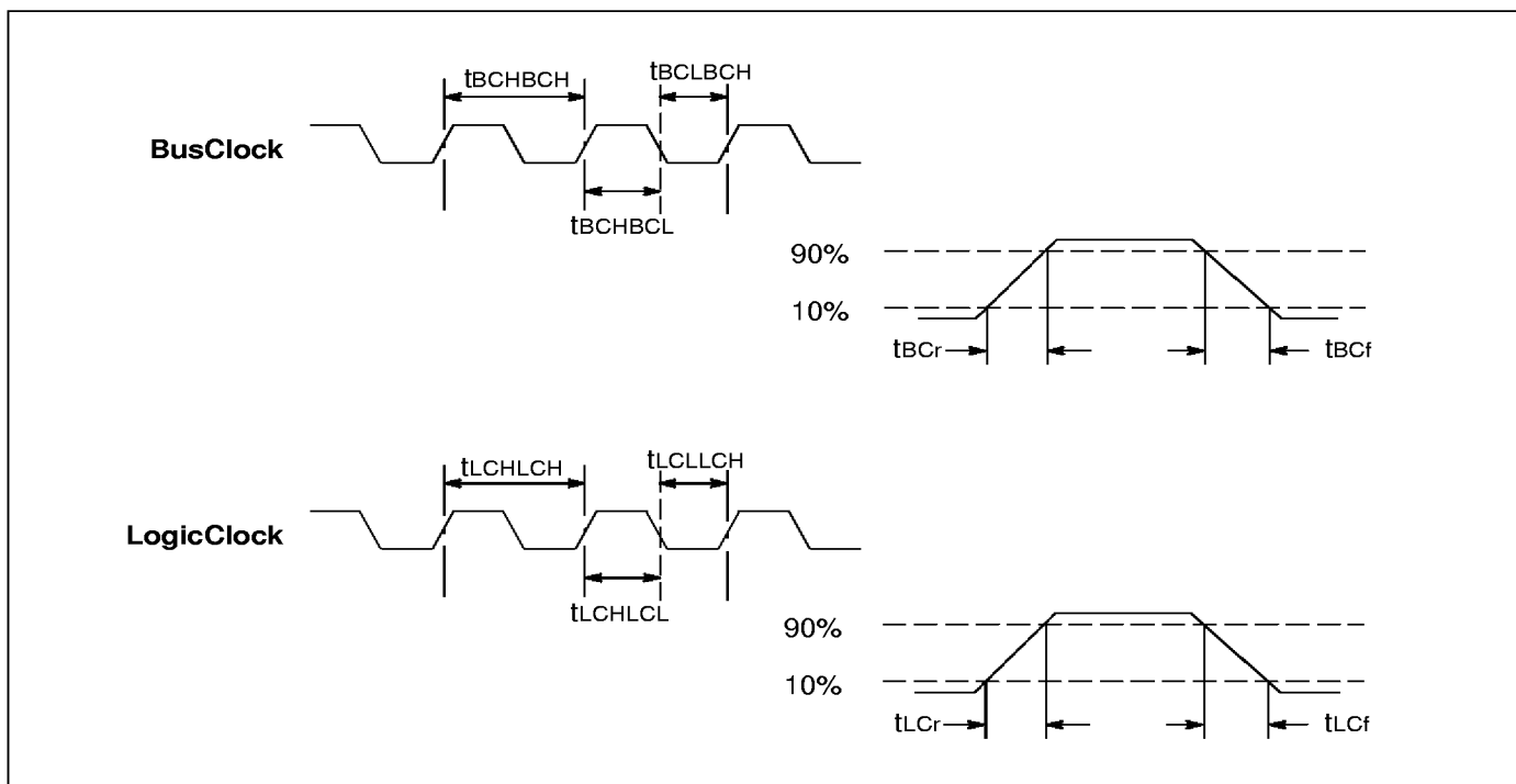
Figure 15.1 BusClock and LogicClock timings
