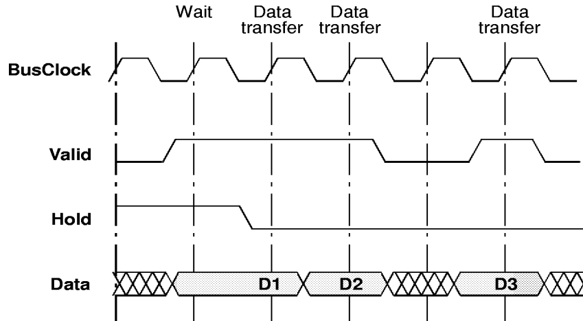
Figure 8.2 Valid/Hold protocol diagram
