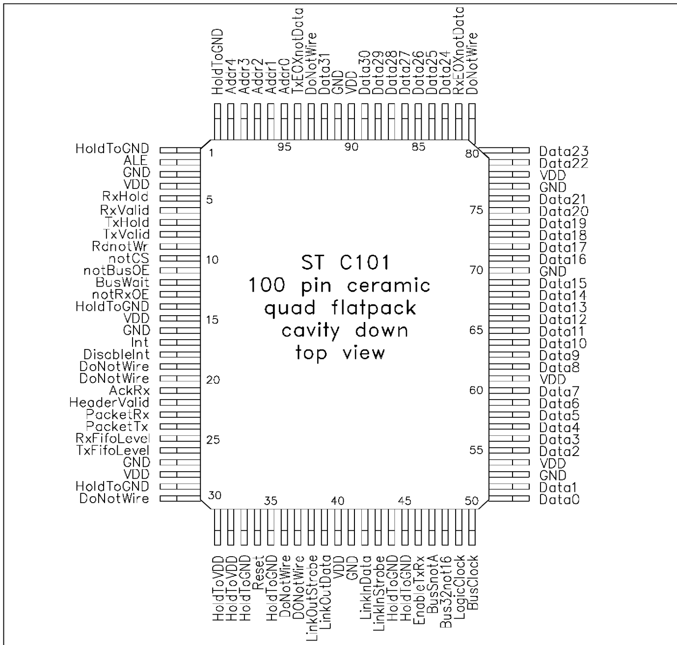
Figure 17.1 STC101 100 pin CQFP package pinout
