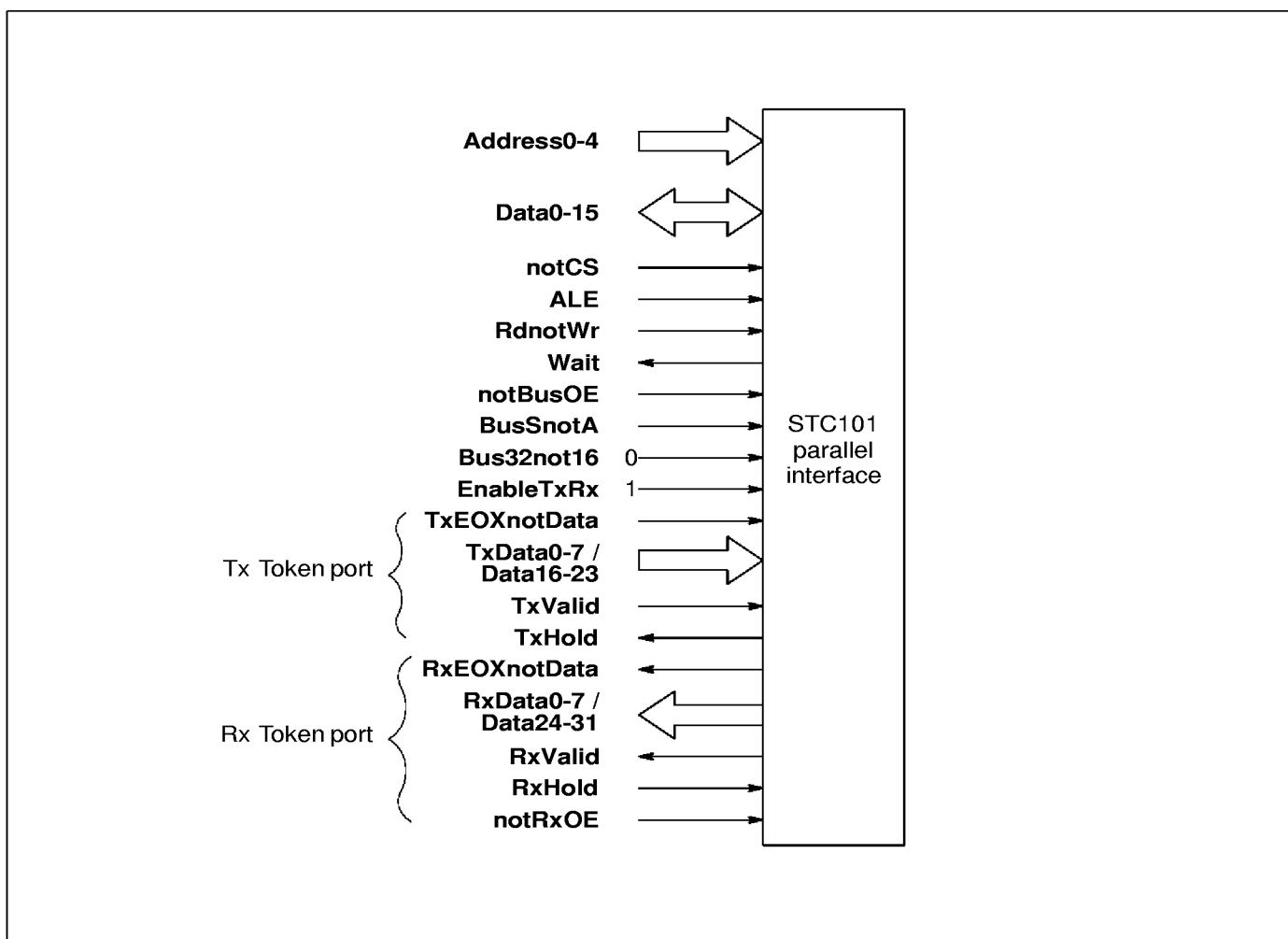
Figure 5.3 16-bit processor interface with token interfaces
