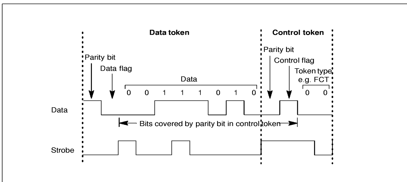
Figure 9.1 Link data and strobe formats
