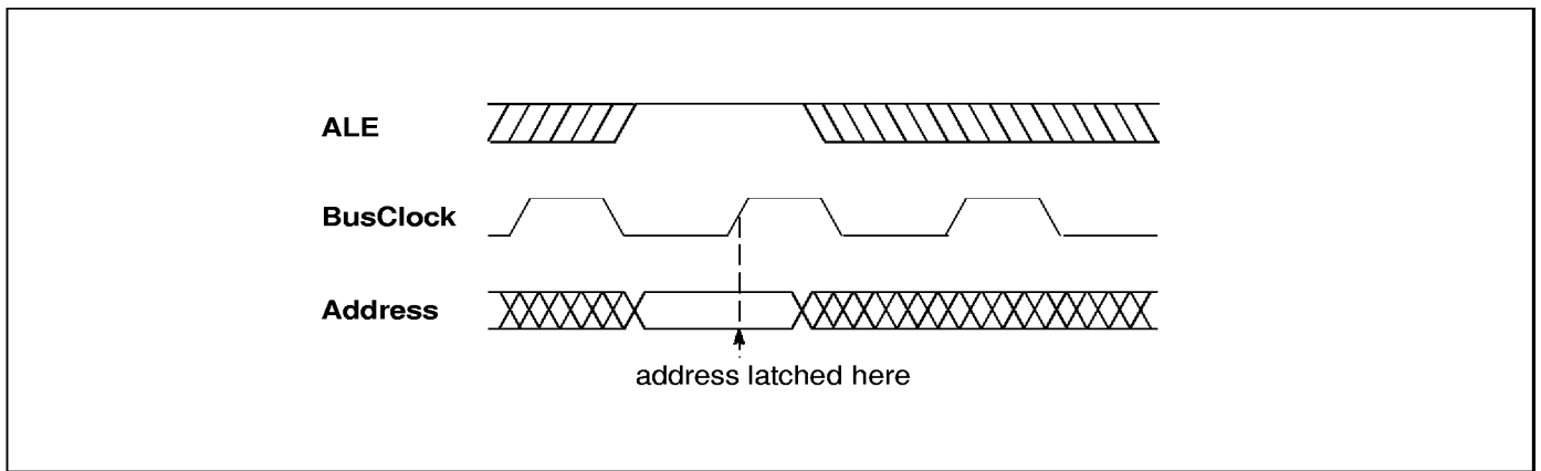
Figure 15.3 Address latching in synchronous mode
