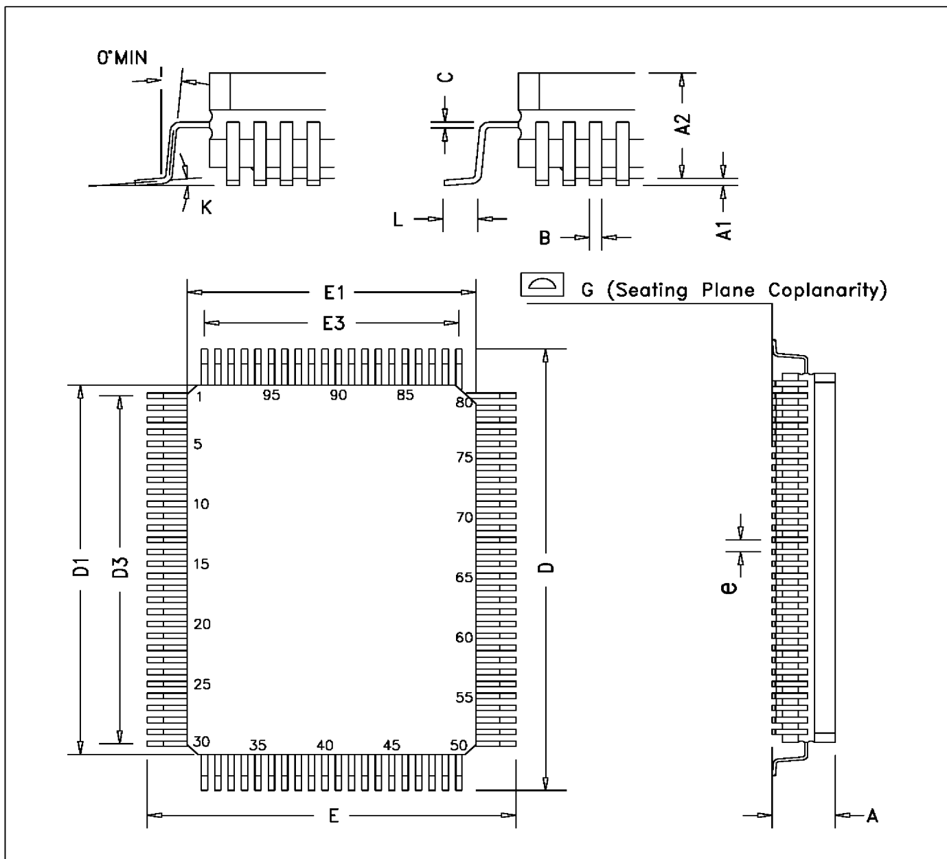
Figure 17.2 STC101 100 pin CQFP package dimensions
