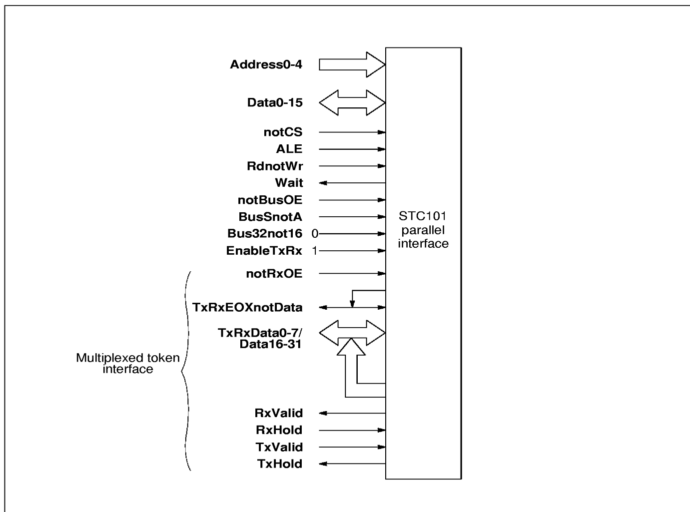
Figure 5.5 16-bit processor interface with multiplexed token interfaces
