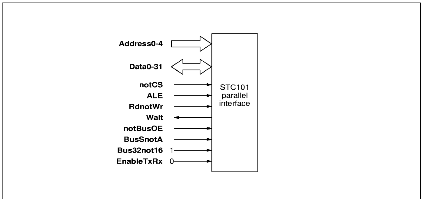
Figure 5.2 32-bit processor interface
