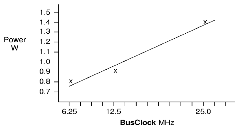
Figure 16.1 Power dissipation vs BusClock frequency
