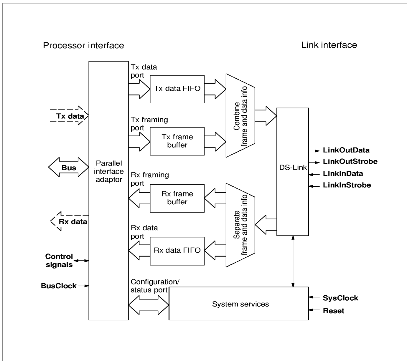
Figure 3.1 STC101 block diagram
