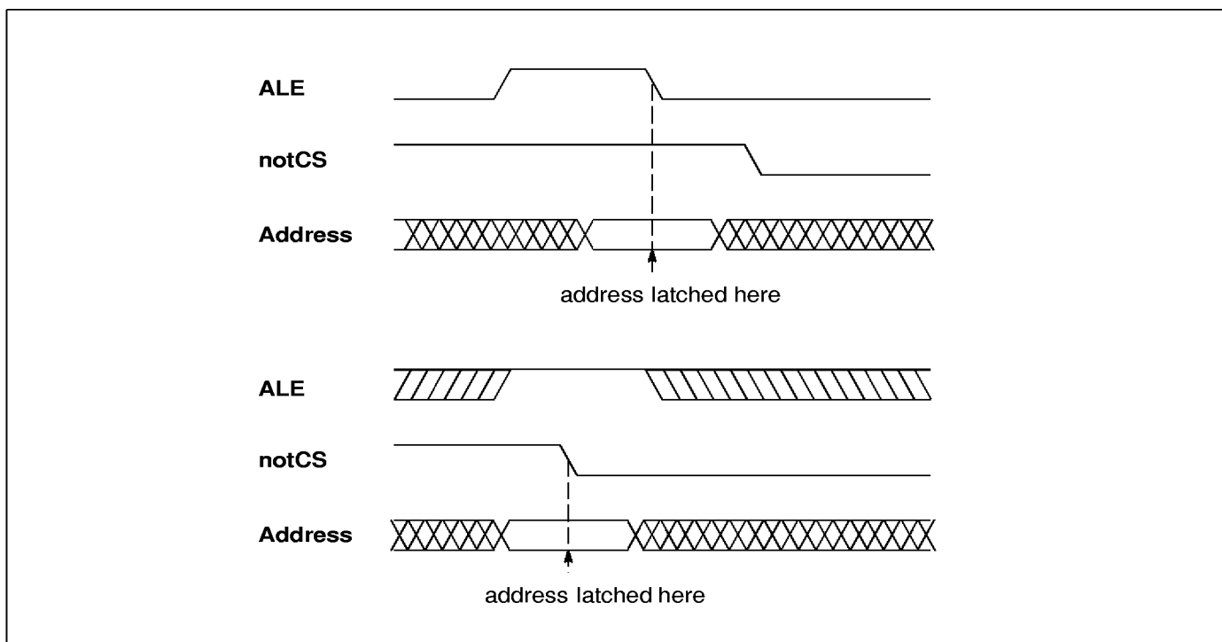
Figure 15.2 Address latching in asynchronous mode
