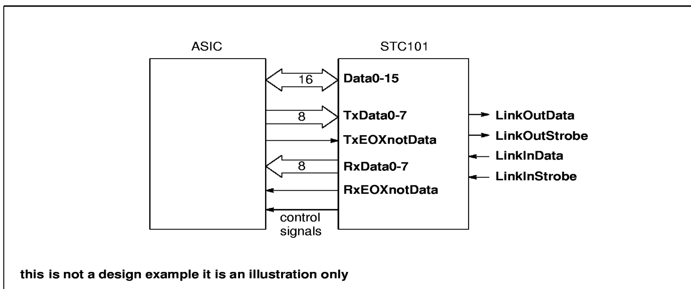
Figure 6.1 Transparent mode
