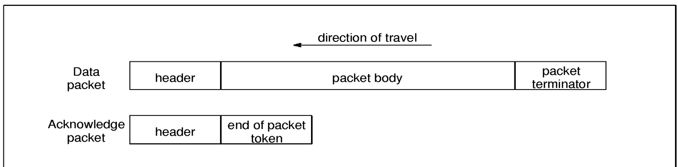
Figure 2.1 Structure of a packet on DS-Links
