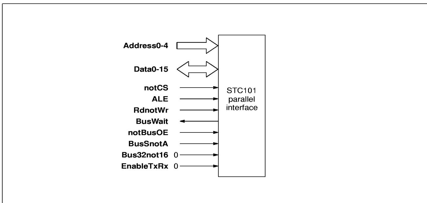
Figure 5.1 16-bit processor interface
