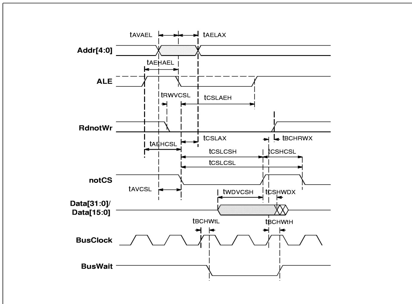
Figure 15.5 Bus interface – asynchronous write cycle
