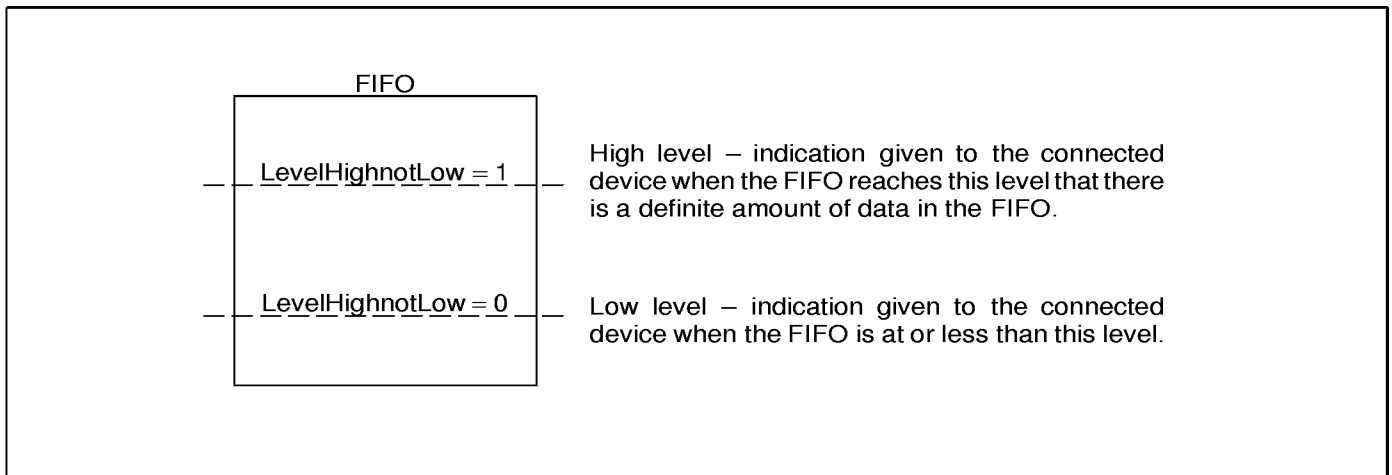
Figure 7.1 Data FIFO programmable levels
