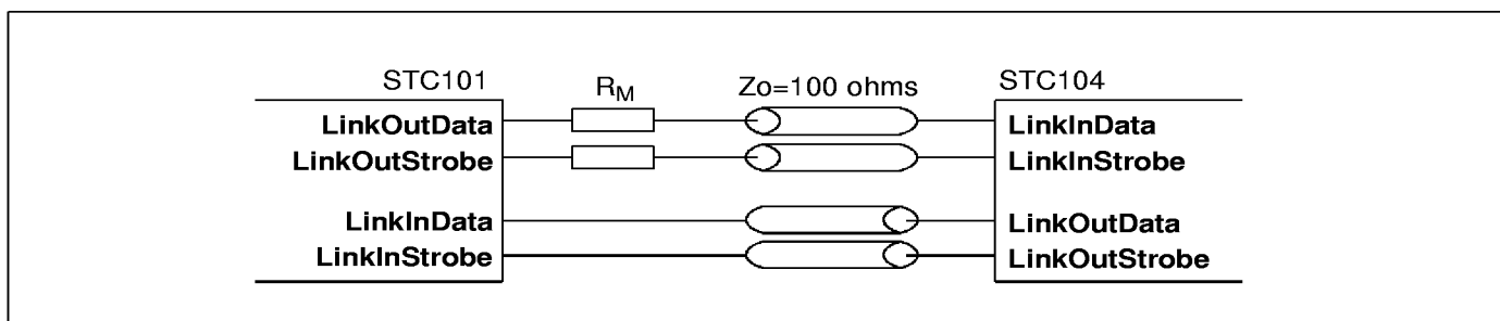
Figure 15.9 DS-Links connected by transmission lines
