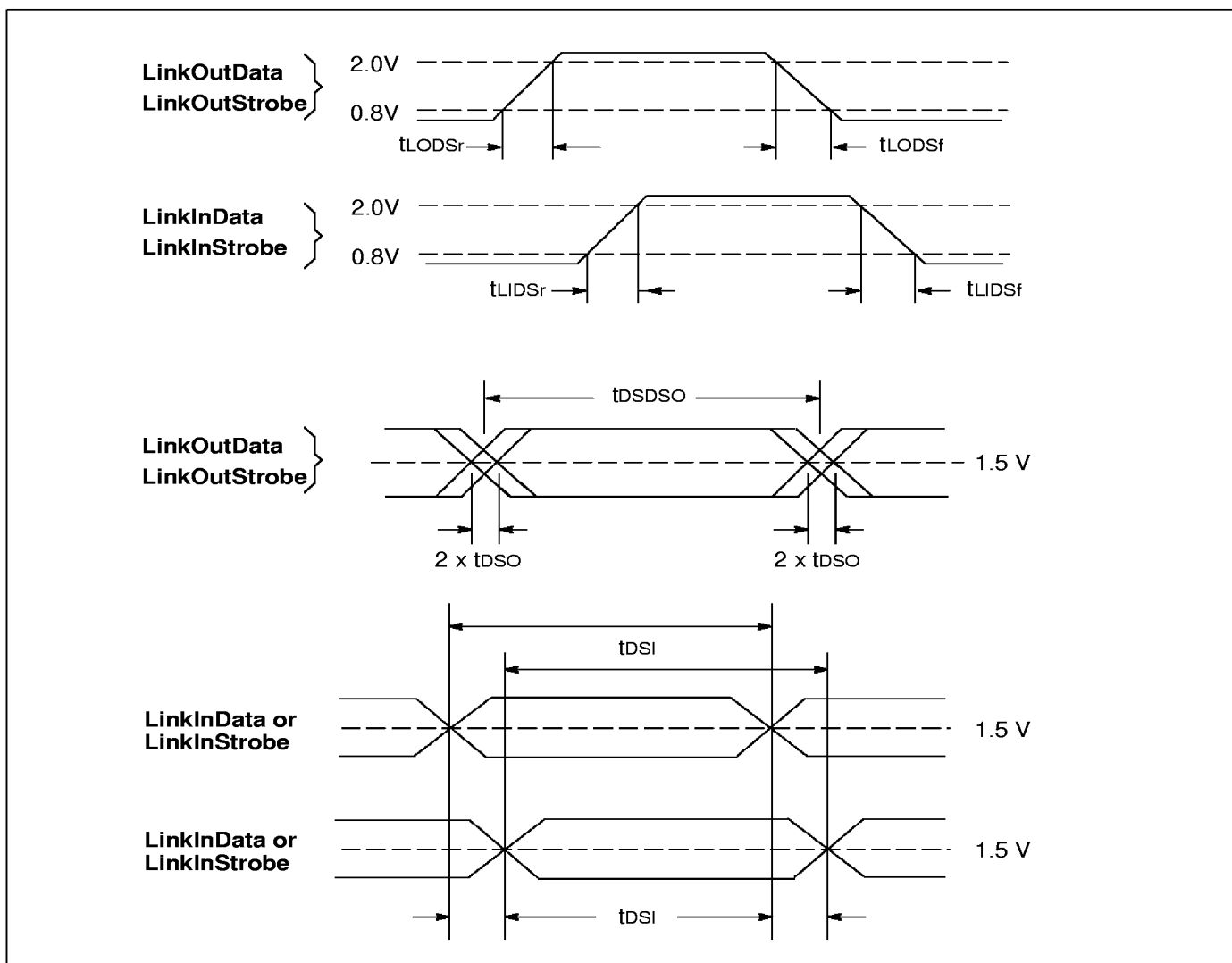
Figure 15.8 DS-Link timing
