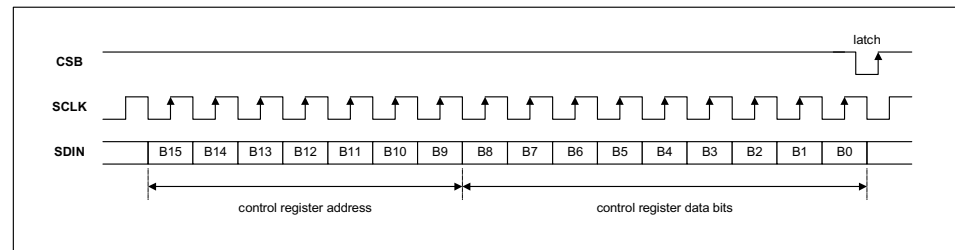
Figure 27 3-Wire Serial Control Interface
