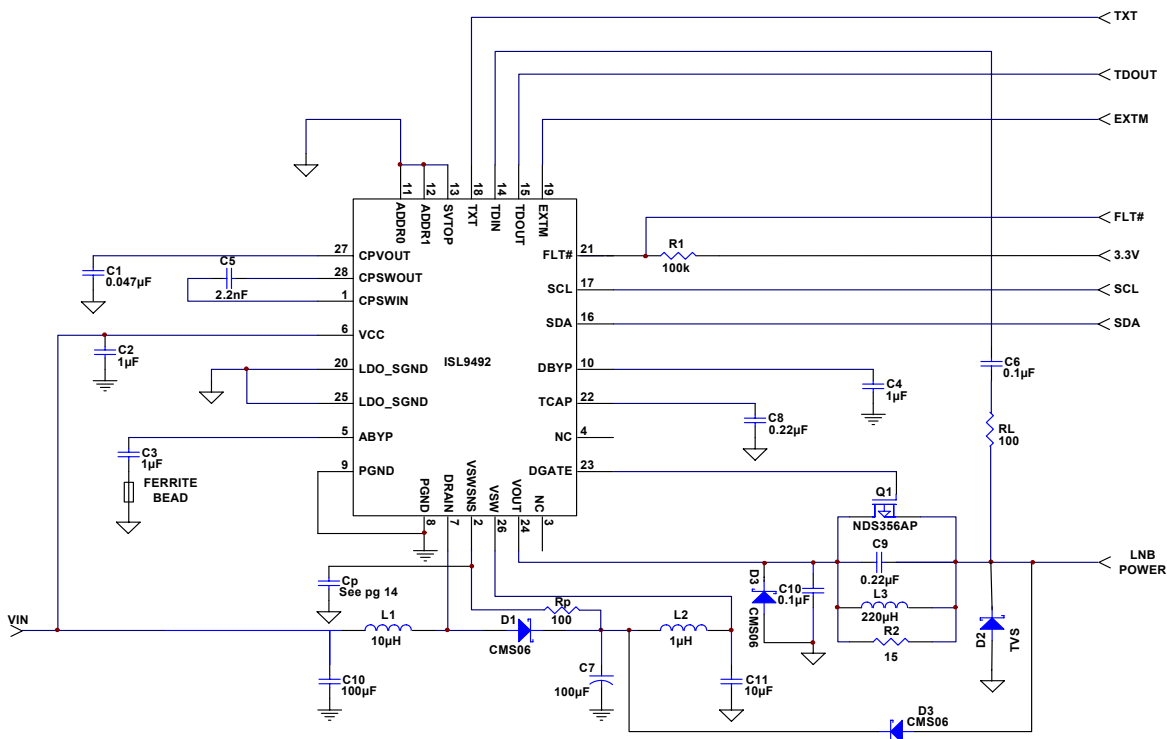
FIGURE 1. TYPICAL APPLICATION
